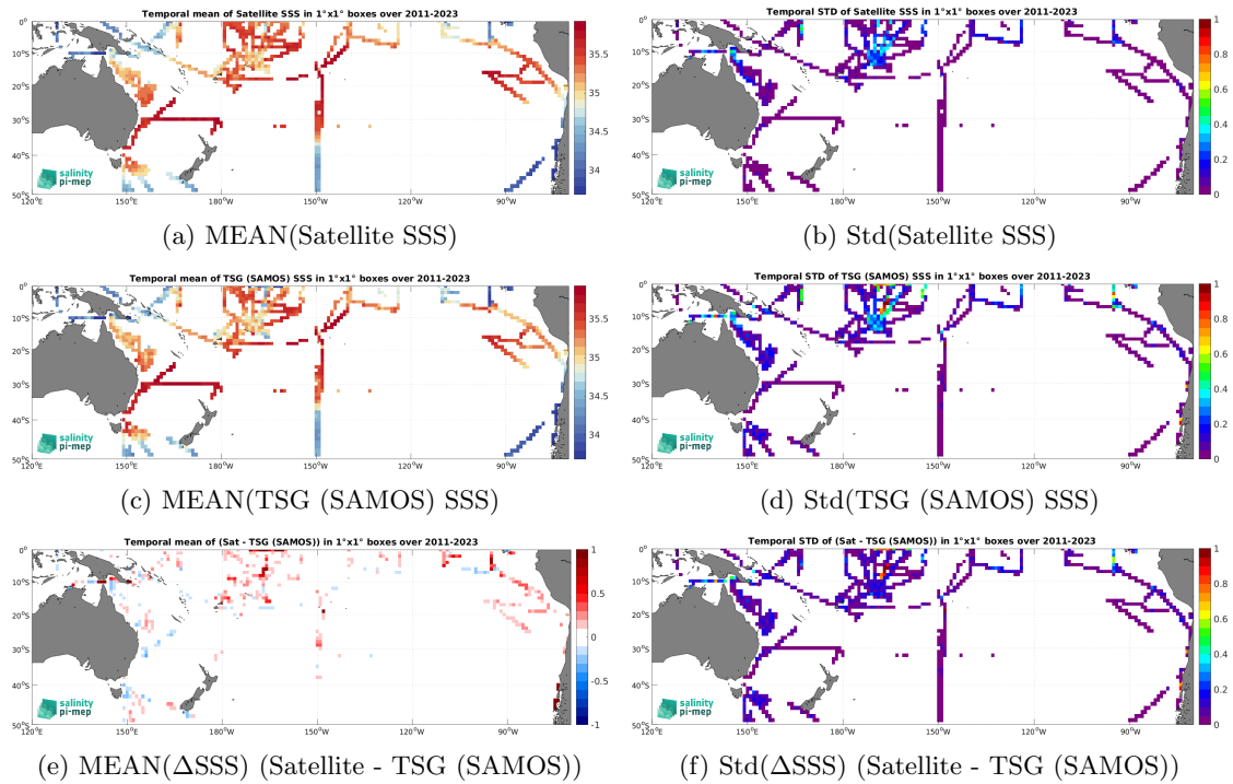
Figure 7: Temporal mean (left) and Std (right) of SSS from SMAP SSS L4 OI v3 - Monthly (ESR) (top), TSG (SAMOS) (middle), and of \Delta SSS (Satellite - TSG (SAMOS)). Only match-up pairs are used to generate these maps.
