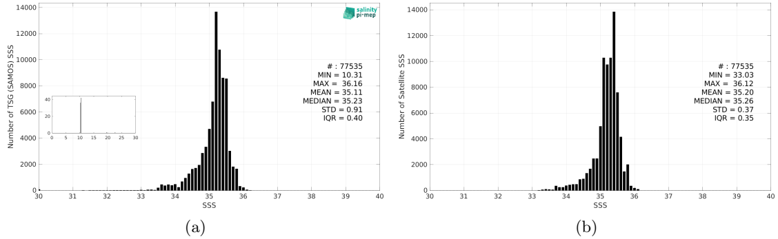
Figure 3: Histograms of SSS from TSG (SAMOS) (a) and SMAP SSS L4 OI v3 - Monthly (ESR) (b) considering all match-up pairs per bins of 0.1 over the South Pacific Ocean Pi-MEP region and for the full satellite product period.
