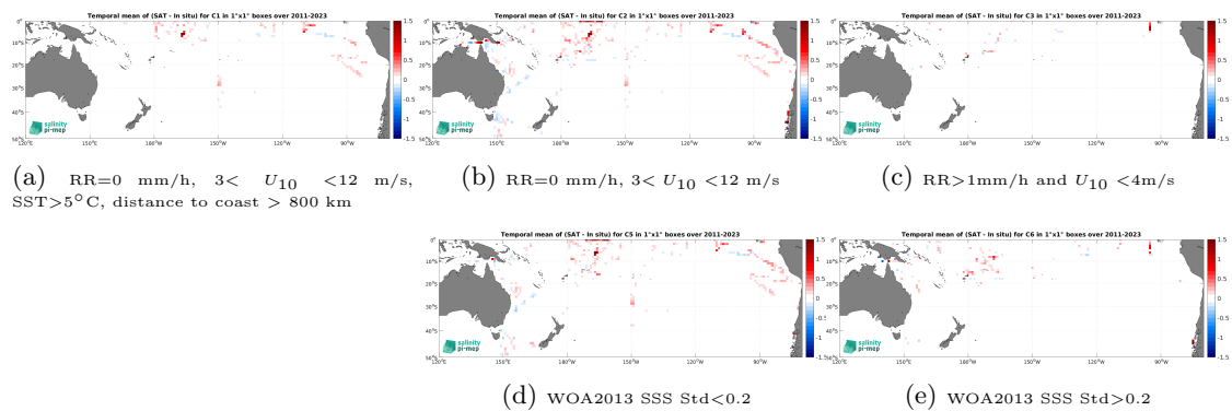
Figure 14: Temporal mean gridded over spatial boxes of size 1^\circ \times 1^\circ of \Delta SSS (SMAP SSS L4 OI v3 - Monthly (ESR) - TSG (SAMOS)) for 5 different subdatasets corresponding to:RR=0 mm/h, 3 < U_{10} < 12 m/s, SST>5°C, distance to coast > 800 km (a), RR=0 mm/h, 3 < U_{10} < 12 m/s (b), RR>1mm/h and U_{10} < 4 m/s (c), WOA2013 SSS Std<0.2 (d), WOA2013 SSS Std>0.2 (e).
