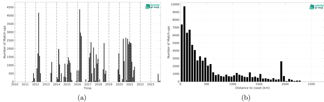
Figure 2: Number of match-ups between TSG (SAMOS) and SMAP SSS L4 OI v3 - Monthly (ESR) SSS as a function of time (a) and as function of the distance to coast (b) over the South Pacific Ocean Pi-MEP region and for the full satellite product period.
