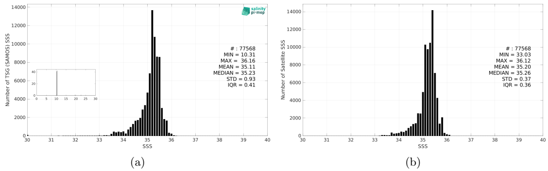
Figure 3: Histograms of SSS from TSG (SAMOS) (a) and SMAP SSS L4 OI v3 - Monthly (ESR) (b) considering all match-up pairs per bins of 0.1 over the South Pacific Ocean Pi-MEP region and for the full satellite product period.
