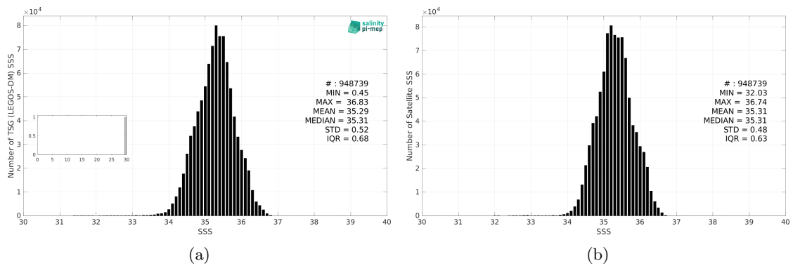
Figure 3: Histograms of SSS from TSG (LEGOS-DM) (a) and SMAP SSS L4 OI v3 - Monthly (ESR) (b) considering all match-up pairs per bins of 0.1 over the South Pacific Ocean Pi-MEP region and for the full satellite product period.
