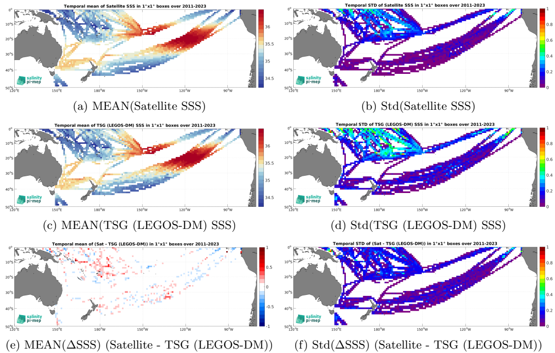
Figure 7: Temporal mean (left) and Std (right) of SSS from SMAP SSS L4 OI v3 - Monthly (ESR) (top), TSG (LEGOS-DM) (middle), and of \Delta SSS (Satellite - TSG (LEGOS-DM)). Only match-up pairs are used to generate these maps.
