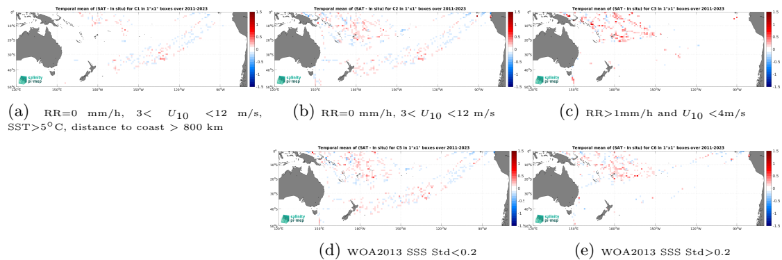
Figure 14: Temporal mean gridded over spatial boxes of size 1^\circ \times 1^\circ of \Delta SSS (SMAP SSS L4 OI v3 - Monthly (ESR) - TSG (LEGOS-DM)) for 5 different subdatasets corresponding to:RR=0 mm/h, 3 < U_{10} < 12 m/s, SST >5^\circ\text{C} , distance to coast > 800 km (a), RR=0 mm/h, 3 < U_{10} < 12 m/s (b), RR >1 mm/h and U_{10} < 4 m/s (c), WOA2013 SSS Std <0.2 (d), WOA2013 SSS Std >0.2 (e).
