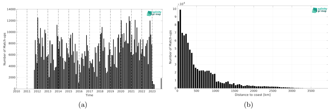
Figure 2: Number of match-ups between TSG (LEGOS-DM) and SMAP SSS L4 OI v3 - Monthly (ESR) SSS as a function of time (a) and as function of the distance to coast (b) over the South Pacific Ocean Pi-MEP region and for the full satellite product period.
