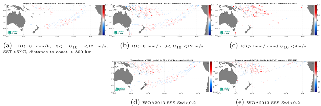
Figure 14: Temporal mean gridded over spatial boxes of size 1^\circ \times 1^\circ of \Delta\text{SSS} (SMAP SSS L4 OI v3 - Monthly (ESR) - TSG (LEGOS-DM)) for 5 different subdatasets corresponding to:RR=0 mm/h, 3 < U_{10} < 12 m/s, SST>5°C, distance to coast > 800 km (a), RR=0 mm/h, 3 < U_{10} < 12 m/s (b), RR>1mm/h and U_{10} < 4 m/s (c), WOA2013 SSS Std<0.2 (d), WOA2013 SSS Std>0.2 (e).
