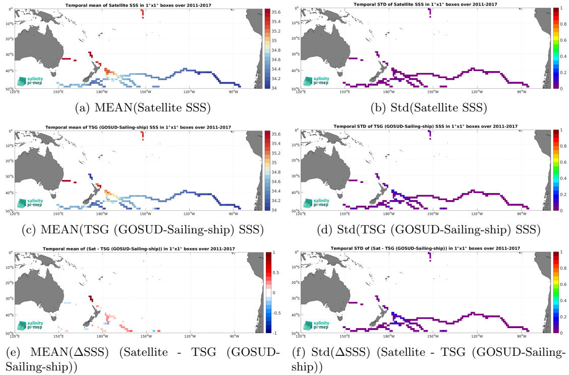
Figure 7: Temporal mean (left) and Std (right) of SSS from SMAP SSS L4 OI v3 - Monthly (ESR) (top), TSG (GOSUD-Sailing-ship) (middle), and of \Delta SSS (Satellite - TSG (GOSUD-Sailing-ship)). Only match-up pairs are used to generate these maps.
