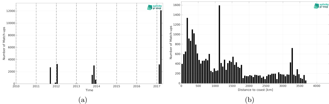
Figure 2: Number of match-ups between TSG (GOSUD-Sailing-ship) and SMAP SSS L4 OI v3 - Monthly (ESR) SSS as a function of time (a) and as function of the distance to coast (b) over the South Pacific Ocean Pi-MEP region and for the full satellite product period.
