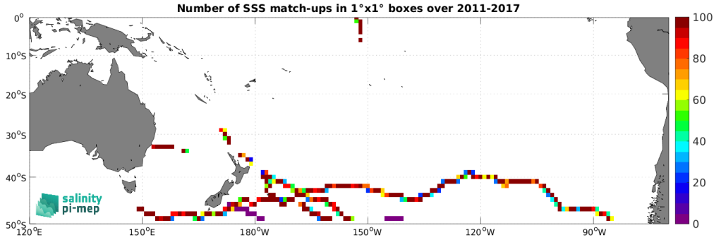
Figure 5: Number of SSS match-ups between TSG (GOSUD-Sailing-ship) SSS and the SMAP SSS L4 OI v3 - Monthly (ESR) SSS product for the South Pacific Ocean Pi-MEP region over 1^\circ \times 1^\circ boxes and for the full satellite product period.
