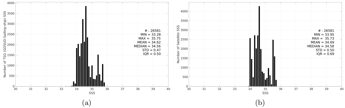
Figure 3: Histograms of SSS from TSG (GOSUD-Sailing-ship) (a) and SMAP SSS L4 OI v3 - Monthly (ESR) (b) considering all match-up pairs per bins of 0.1 over the South Pacific Ocean Pi-MEP region and for the full satellite product period.
