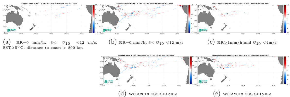
Figure 14: Temporal mean gridded over spatial boxes of size 1^\circ \times 1^\circ of \Delta\text{SSS} (SMAP SSS L4 OI v3 - Monthly (ESR) - TSG (GOSUD-Research-vessel)) for 5 different subdatasets corresponding to:RR=0 mm/h, 3 < U_{10} < 12 m/s, SST>5°C, distance to coast > 800 km (a), RR=0 mm/h, 3 < U_{10} < 12 m/s (b), RR>1mm/h and U_{10} < 4 m/s (c), WOA2013 SSS Std<0.2 (d), WOA2013 SSS Std>0.2 (e).
