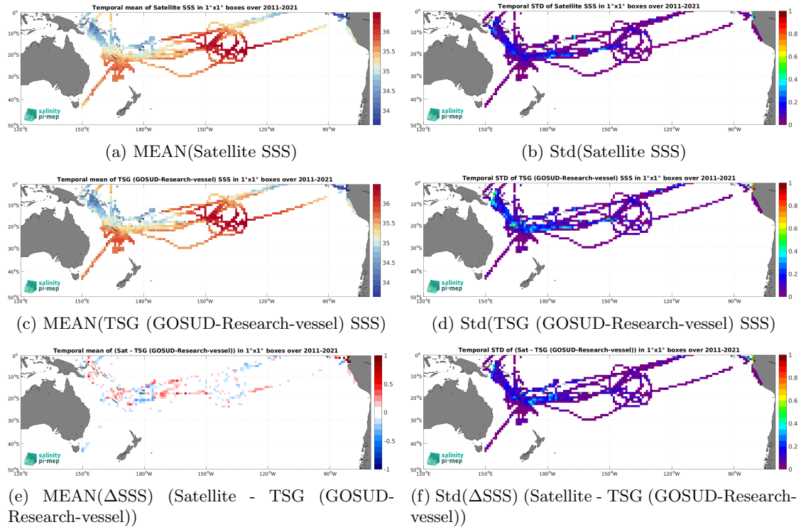
Figure 7: Temporal mean (left) and Std (right) of SSS from SMAP SSS L4 OI v3 - Monthly (ESR) (top), TSG (GOSUD-Research-vessel) (middle), and of \Delta SSS (Satellite - TSG (GOSUD-Research-vessel)). Only match-up pairs are used to generate these maps.
