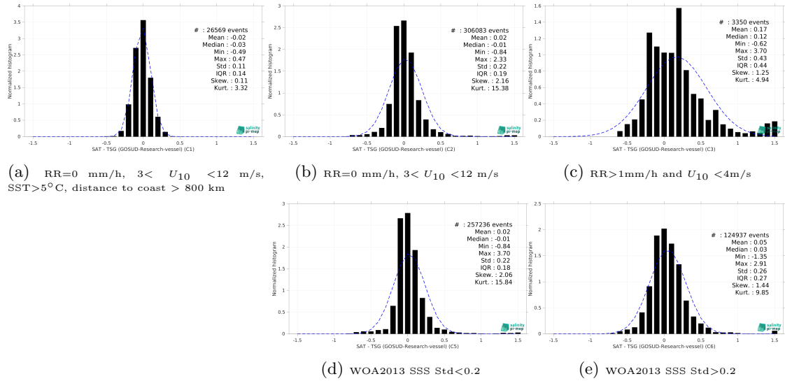
Figure 15: Normalized histogram of \Delta\text{SSS} (SMAP SSS L4 OI v3 - Monthly (ESR) - TSG (GOSUD-Research-vessel)) for 5 different subdatasets corresponding to: RR=0 mm/h, 3 < U_{10} < 12 m/s, SST>5°C, distance to coast > 800 km (a), RR=0 mm/h, 3 < U_{10} < 12 m/s (b), RR>1mm/h and U_{10} < 4 m/s (c), WOA2013 SSS Std<0.2 (d), WOA2013 SSS Std>0.2 (e).
