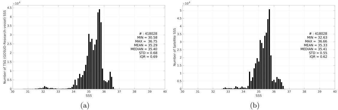
Figure 3: Histograms of SSS from TSG (GOSUD-Research-vessel) (a) and SMAP SSS L4 OI v3 - Monthly (ESR) (b) considering all match-up pairs per bins of 0.1 over the South Pacific Ocean Pi-MEP region and for the full satellite product period.
