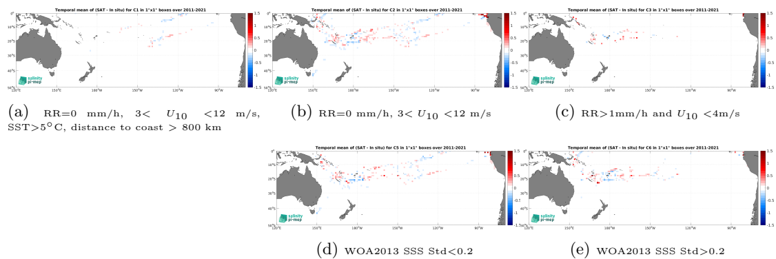
Figure 14: Temporal mean gridded over spatial boxes of size 1^\circ \times 1^\circ of \Delta SSS (SMAP SSS L4 OI v3 - Monthly (ESR) - TSG (GOSUD-Research-vessel)) for 5 different subdatasets corresponding to:RR=0 mm/h, 3 < U_{10} < 12 m/s, SST >5^\circ\text{C} , distance to coast > 800 km (a), RR=0 mm/h, 3 < U_{10} < 12 m/s (b), RR >1 mm/h and U_{10} < 4 m/s (c), WOA2013 SSS Std <0.2 (d), WOA2013 SSS Std >0.2 (e).
