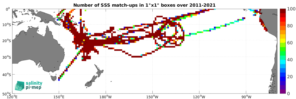
Figure 5: Number of SSS match-ups between TSG (GOSUD-Research-vessel) SSS and the SMAP SSS L4 OI v3 - Monthly (ESR) SSS product for the South Pacific Ocean Pi-MEP region over 1^\circ \times 1^\circ boxes and for the full satellite product period.
