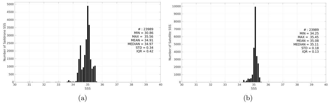
Figure 3: Histograms of SSS from Saildrone (a) and SMAP SSS L4 OI v3 - Monthly (ESR) (b) considering all match-up pairs per bins of 0.1 over the South Pacific Ocean Pi-MEP region and for the full satellite product period.
