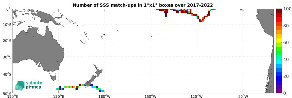
Figure 5: Number of SSS match-ups between Saildrone SSS and the SMAP SSS L4 OI v3 - Monthly (ESR) SSS product for the South Pacific Ocean Pi-MEP region over 1^\circ \times 1^\circ boxes and for the full satellite product period.
