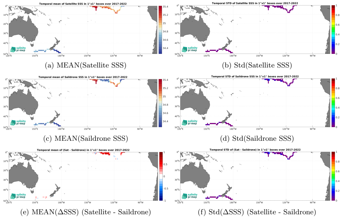
Figure 7: Temporal mean (left) and Std (right) of SSS from SMAP SSS L4 OI v3 - Monthly (ESR) (top), Saildrone (middle), and of \Delta SSS (Satellite - Saildrone). Only match-up pairs are used to generate these maps.
