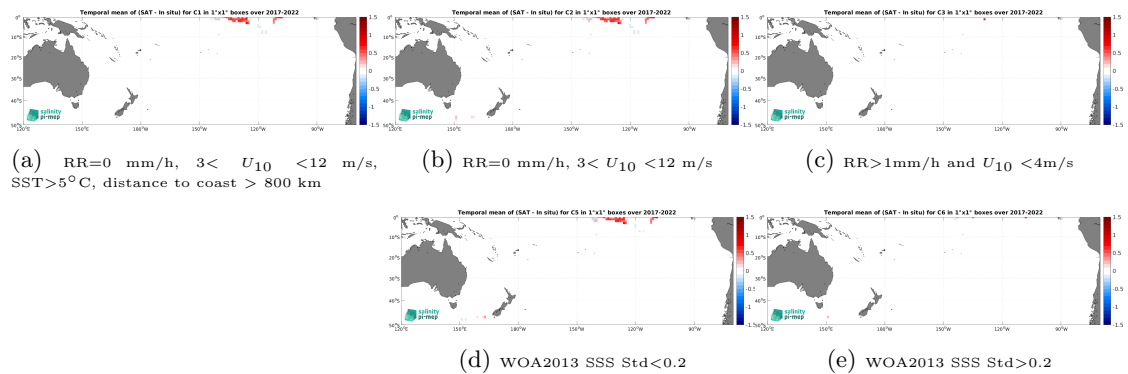
Figure 14: Temporal mean gridded over spatial boxes of size 1^\circ \times 1^\circ of \Delta\text{SSS} (SMAP SSS L4 OI v3 - Monthly (ESR) - Saildrone) for 5 different subdatasets corresponding to:RR=0 mm/h, 3 < U_{10} < 12 m/s, SST>5°C, distance to coast > 800 km (a), RR=0 mm/h, 3 < U_{10} < 12 m/s (b), RR>1mm/h and U_{10} < 4 m/s (c), WOA2013 SSS Std<0.2 (d), WOA2013 SSS Std>0.2 (e).
