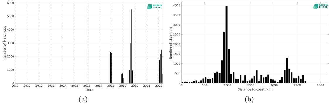
Figure 2: Number of match-ups between Saildrone and SMAP SSS L4 OI v3 - Monthly (ESR) SSS as a function of time (a) and as function of the distance to coast (b) over the South Pacific Ocean Pi-MEP region and for the full satellite product period.
