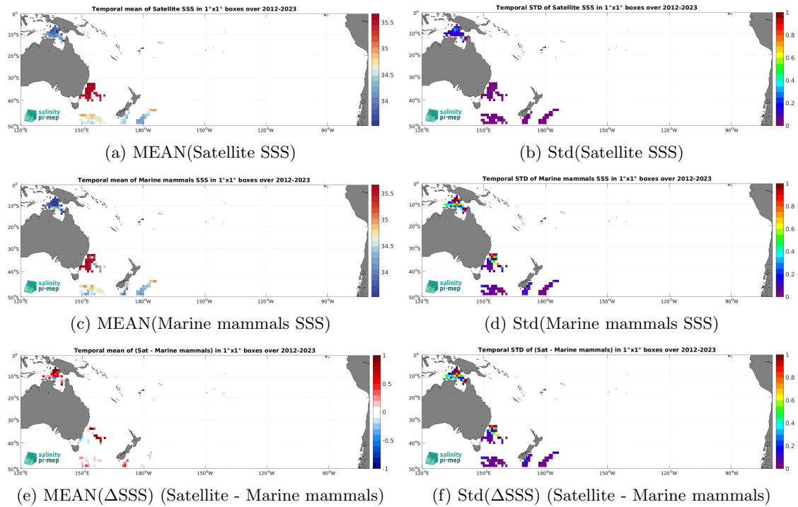
Figure 7: Temporal mean (left) and Std (right) of SSS from SMAP SSS L4 OI v3 - Monthly (ESR) (top), Marine mammals (middle), and of \Delta SSS (Satellite - Marine mammals). Only match-up pairs are used to generate these maps.
