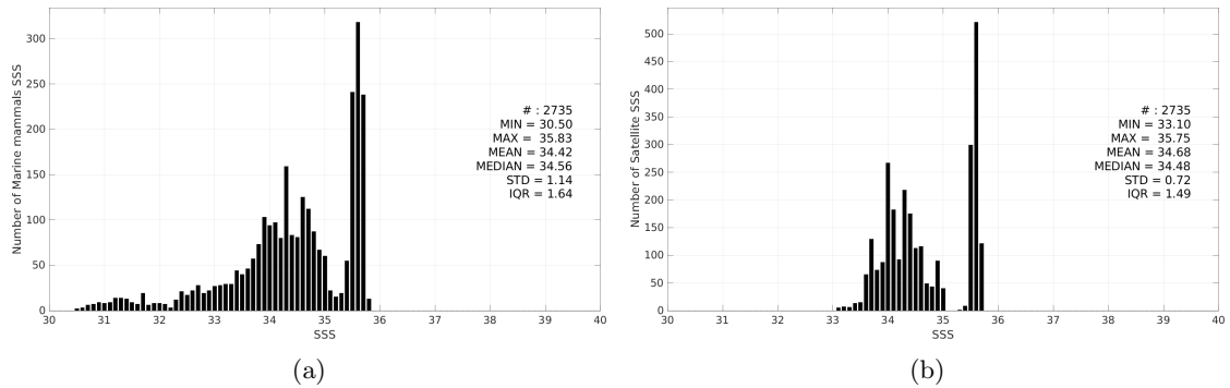
Figure 3: Histograms of SSS from Marine mammals (a) and SMAP SSS L4 OI v3 - Monthly (ESR) (b) considering all match-up pairs per bins of 0.1 over the South Pacific Ocean Pi-MEP region and for the full satellite product period.
