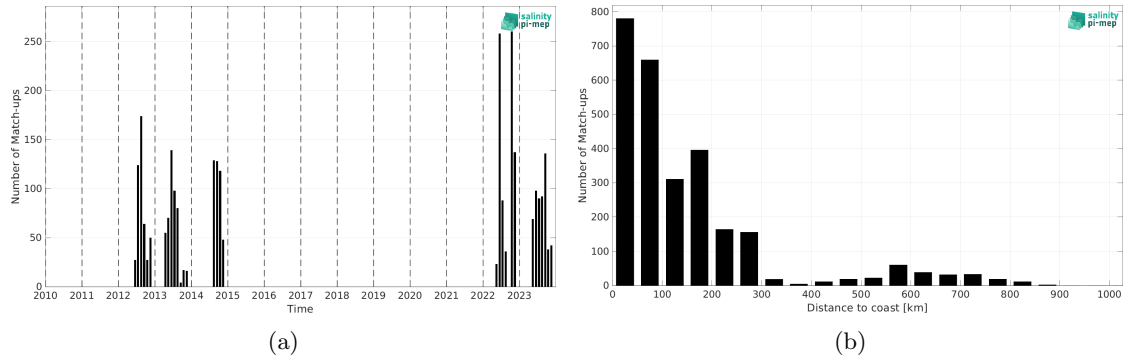
Figure 2: Number of match-ups between Marine mammals and SMAP SSS L4 OI v3 - Monthly (ESR) SSS as a function of time (a) and as function of the distance to coast (b) over the South Pacific Ocean Pi-MEP region and for the full satellite product period.
