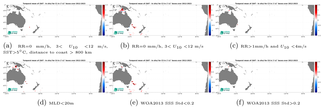
Figure 14: Temporal mean gridded over spatial boxes of size 1^\circ \times 1^\circ of \Delta SSS (SMAP SSS L4 OI v3 - Monthly (ESR) - Marine mammals) for 6 different subdatasets corresponding to:RR=0 mm/h, 3 < U_{10} < 12 m/s, SST >5^\circ C, distance to coast > 800 km (a), RR=0 mm/h, 3 < U_{10} < 12 m/s (b), RR >1 mm/h and U_{10} < 4 m/s (c),MLD <20 m (d),WOA2013 SSS Std <0.2 (e),WOA2013 SSS Std >0.2 (f).
