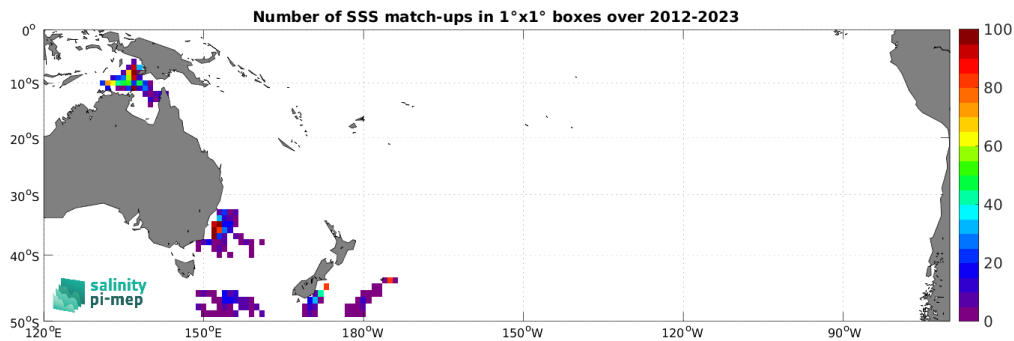
Figure 5: Number of SSS match-ups between Marine mammals SSS and the SMAP SSS L4 OI v3 - Monthly (ESR) SSS product for the South Pacific Ocean Pi-MEP region over 1^\circ \times 1^\circ boxes and for the full satellite product period.
