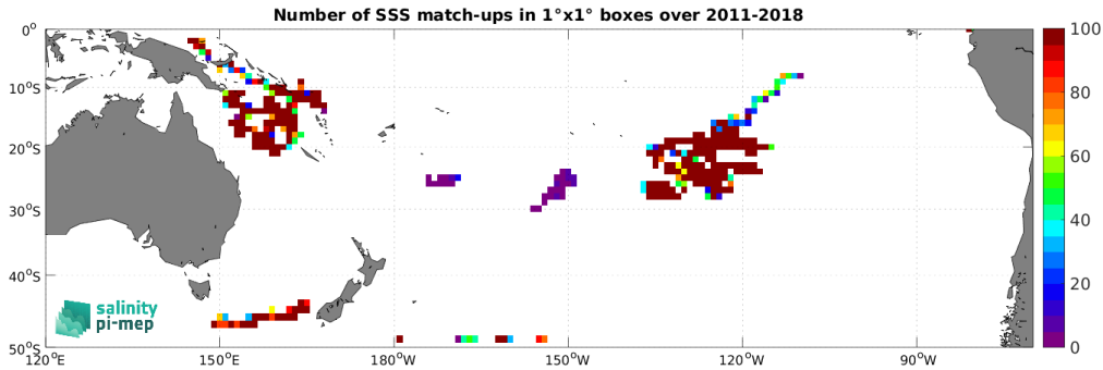
Figure 4: Number of SSS match-ups between Surface drifters SSS and the SMAP SSS L4 OI v3 - Monthly (ESR) SSS product for the South Pacific Ocean Pi-MEP region over 1^\circ \times 1^\circ boxes and for the full satellite product period.
