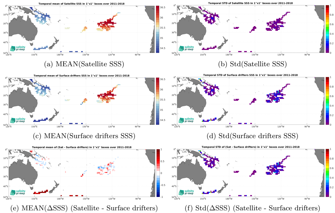
Figure 6: Temporal mean (left) and Std (right) of SSS from SMAP SSS L4 OI v3 - Monthly (ESR) (top), Surface drifters (middle), and of \Delta SSS (Satellite - Surface drifters). Only match-up pairs are used to generate these maps.
