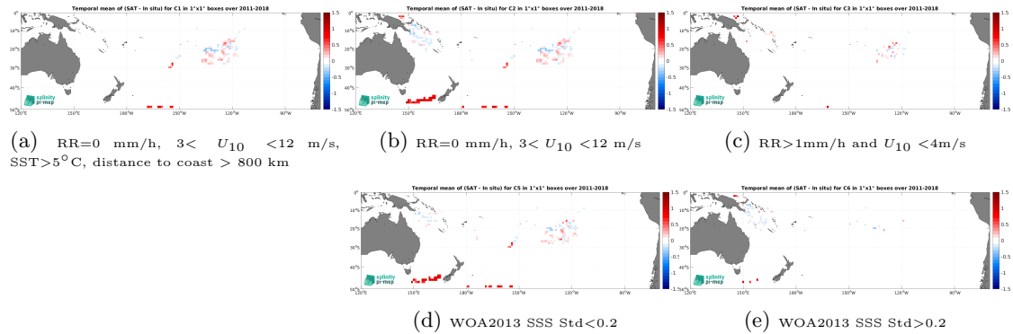
Figure 13: Temporal mean gridded over spatial boxes of size 1^\circ \times 1^\circ of \Delta SSS (SMAP SSS L4 OI v3 - Monthly (ESR) - Surface drifters) for 5 different subdatasets corresponding to:RR=0 mm/h, 3 < U_{10} < 12 m/s, SST >5^\circ\text{C} , distance to coast > 800 km (a), RR=0 mm/h, 3 < U_{10} < 12 m/s (b), RR >1 mm/h and U_{10} < 4 m/s (c), WOA2013 SSS Std <0.2 (d), WOA2013 SSS Std >0.2 (e).
