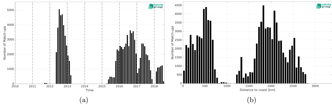
Figure 2: Number of match-ups between Surface drifters and SMAP SSS L4 OI v3 - Monthly (ESR) SSS as a function of time (a) and as function of the distance to coast (b) over the South Pacific Ocean Pi-MEP region and for the full satellite product period.
