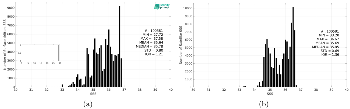
Figure 3: Histograms of SSS from Surface drifters (a) and SMAP SSS L4 OI v3 - Monthly (ESR) (b) considering all match-up pairs per bins of 0.1 over the South Pacific Ocean Pi-MEP region and for the full satellite product period.
