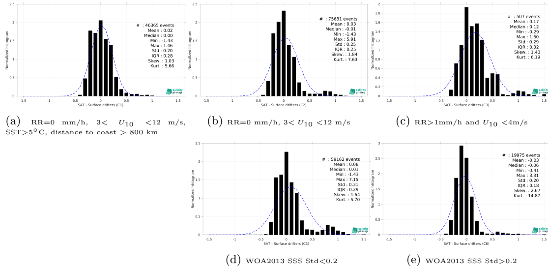
Figure 14: Normalized histogram of \Delta\text{SSS} (SMAP SSS L4 OI v3 - Monthly (ESR) - Surface drifters) for 5 different subdatasets corresponding to: RR=0 mm/h, 3 < U_{10} < 12 m/s, SST>5°C, distance to coast > 800 km (a), RR=0 mm/h, 3 < U_{10} < 12 m/s (b), RR>1mm/h and U_{10} < 4 m/s (c), WOA2013 SSS Std<0.2 (d), WOA2013 SSS Std>0.2 (e).
