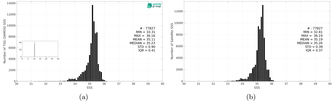
Figure 3: Histograms of SSS from TSG (SAMOS) (a) and SMAP SSS L4 OI v3 - Daily (ESR) (b) considering all match-up pairs per bins of 0.1 over the South Pacific Ocean Pi-MEP region and for the full satellite product period.
