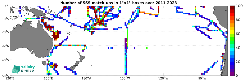
Figure 5: Number of SSS match-ups between TSG (SAMOS) SSS and the SMAP SSS L4 OI v3 - Daily (ESR) SSS product for the South Pacific Ocean Pi-MEP region over 1^\circ \times 1^\circ boxes and for the full satellite product period.
