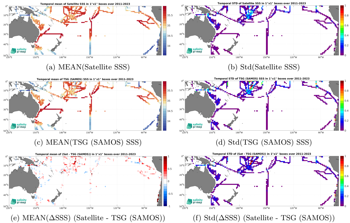
Figure 7: Temporal mean (left) and Std (right) of SSS from SMAP SSS L4 OI v3 - Daily (ESR) (top), TSG (SAMOS) (middle), and of \Delta SSS (Satellite - TSG (SAMOS)). Only match-up pairs are used to generate these maps.
