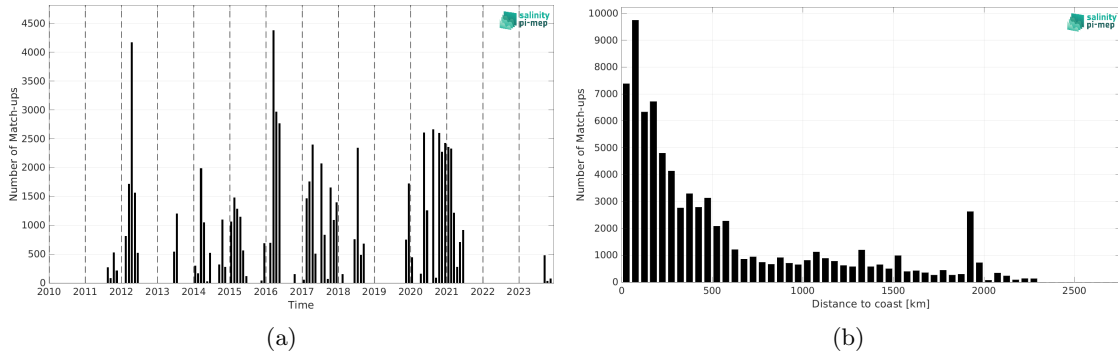
Figure 2: Number of match-ups between TSG (SAMOS) and SMAP SSS L4 OI v3 - Daily (ESR) SSS as a function of time (a) and as function of the distance to coast (b) over the South Pacific Ocean Pi-MEP region and for the full satellite product period.
