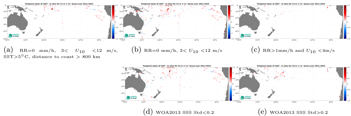
Figure 14: Temporal mean gridded over spatial boxes of size 1^\circ \times 1^\circ of \Delta SSS (SMAP SSS L4 OI v3 - Daily (ESR) - TSG (SAMOS)) for 5 different subdatasets corresponding to:RR=0 mm/h, 3 < U_{10} < 12 m/s, SST >5^\circ\text{C} , distance to coast > 800 km (a), RR=0 mm/h, 3 < U_{10} < 12 m/s (b), RR >1 mm/h and U_{10} < 4 m/s (c), WOA2013 SSS Std <0.2 (d), WOA2013 SSS Std >0.2 (e).
