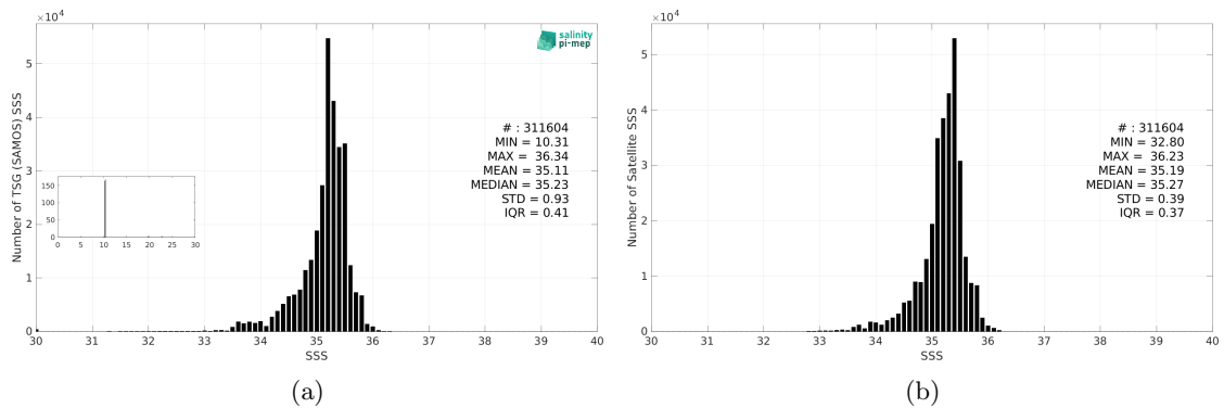
Figure 3: Histograms of SSS from TSG (SAMOS) (a) and SMAP SSS L4 OI v3 - Daily (ESR) (b) considering all match-up pairs per bins of 0.1 over the South Pacific Ocean Pi-MEP region and for the full satellite product period.
