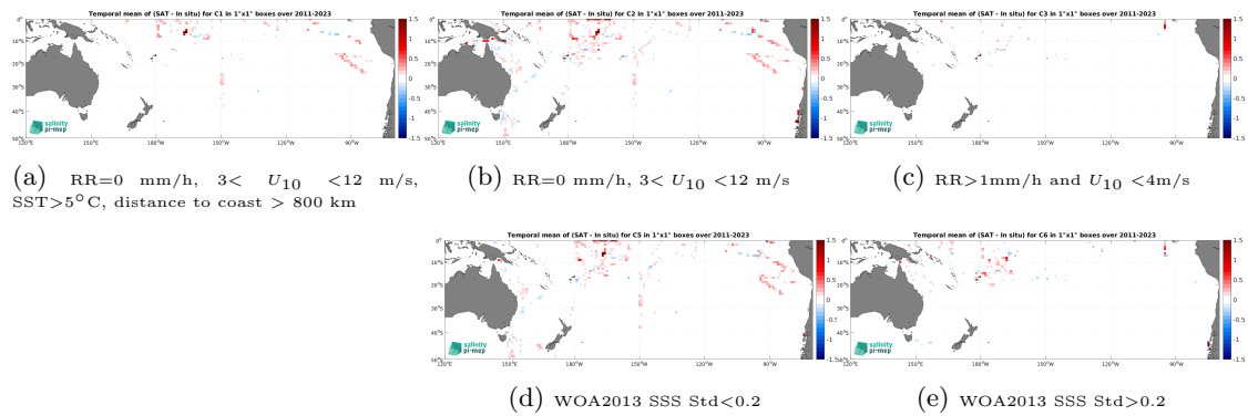
Figure 14: Temporal mean gridded over spatial boxes of size 1^\circ \times 1^\circ of \Delta\text{SSS} (SMAP SSS L4 OI v3 - Daily (ESR) - TSG (SAMOS)) for 5 different subdatasets corresponding to:RR=0 mm/h, 3 < U_{10} < 12 m/s, SST>5°C, distance to coast > 800 km (a), RR=0 mm/h, 3 < U_{10} < 12 m/s (b), RR>1mm/h and U_{10} < 4 m/s (c), WOA2013 SSS Std<0.2 (d), WOA2013 SSS Std>0.2 (e).
