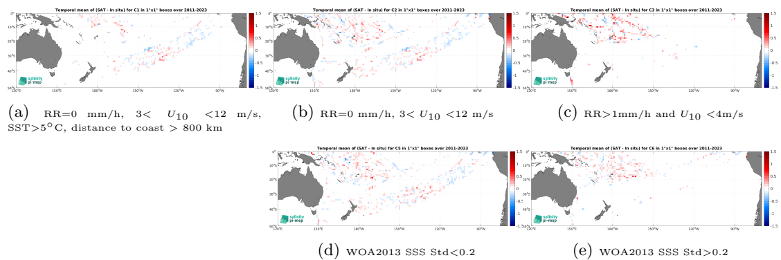
Figure 14: Temporal mean gridded over spatial boxes of size 1^\circ \times 1^\circ of \Delta SSS (SMAP SSS L4 OI v3 - Daily (ESR) - TSG (LEGOS-DM)) for 5 different subdatasets corresponding to:RR=0 mm/h, 3 < U_{10} < 12 m/s, SST >5^\circ\text{C} , distance to coast > 800 km (a), RR=0 mm/h, 3 < U_{10} < 12 m/s (b), RR >1 mm/h and U_{10} < 4 m/s (c), WOA2013 SSS Std <0.2 (d), WOA2013 SSS Std >0.2 (e).
