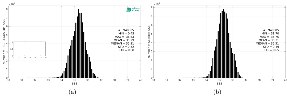
Figure 3: Histograms of SSS from TSG (LEGOS-DM) (a) and SMAP SSS L4 OI v3 - Daily (ESR) (b) considering all match-up pairs per bins of 0.1 over the South Pacific Ocean Pi-MEP region and for the full satellite product period.
