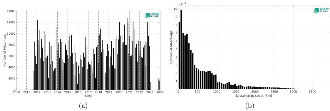
Figure 2: Number of match-ups between TSG (LEGOS-DM) and SMAP SSS L4 OI v3 - Daily (ESR) SSS as a function of time (a) and as function of the distance to coast (b) over the South Pacific Ocean Pi-MEP region and for the full satellite product period.
