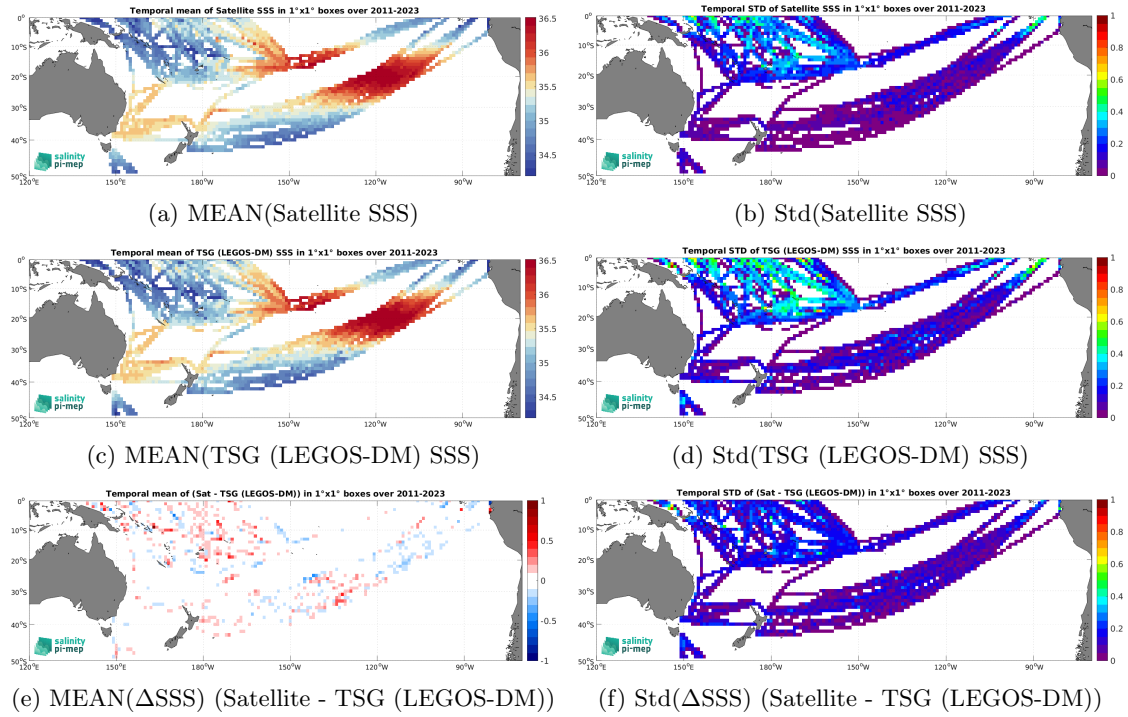
Figure 7: Temporal mean (left) and Std (right) of SSS from SMAP SSS L4 OI v3 - Daily (ESR) (top), TSG (LEGOS-DM) (middle), and of \Delta SSS (Satellite - TSG (LEGOS-DM)). Only match-up pairs are used to generate these maps.
