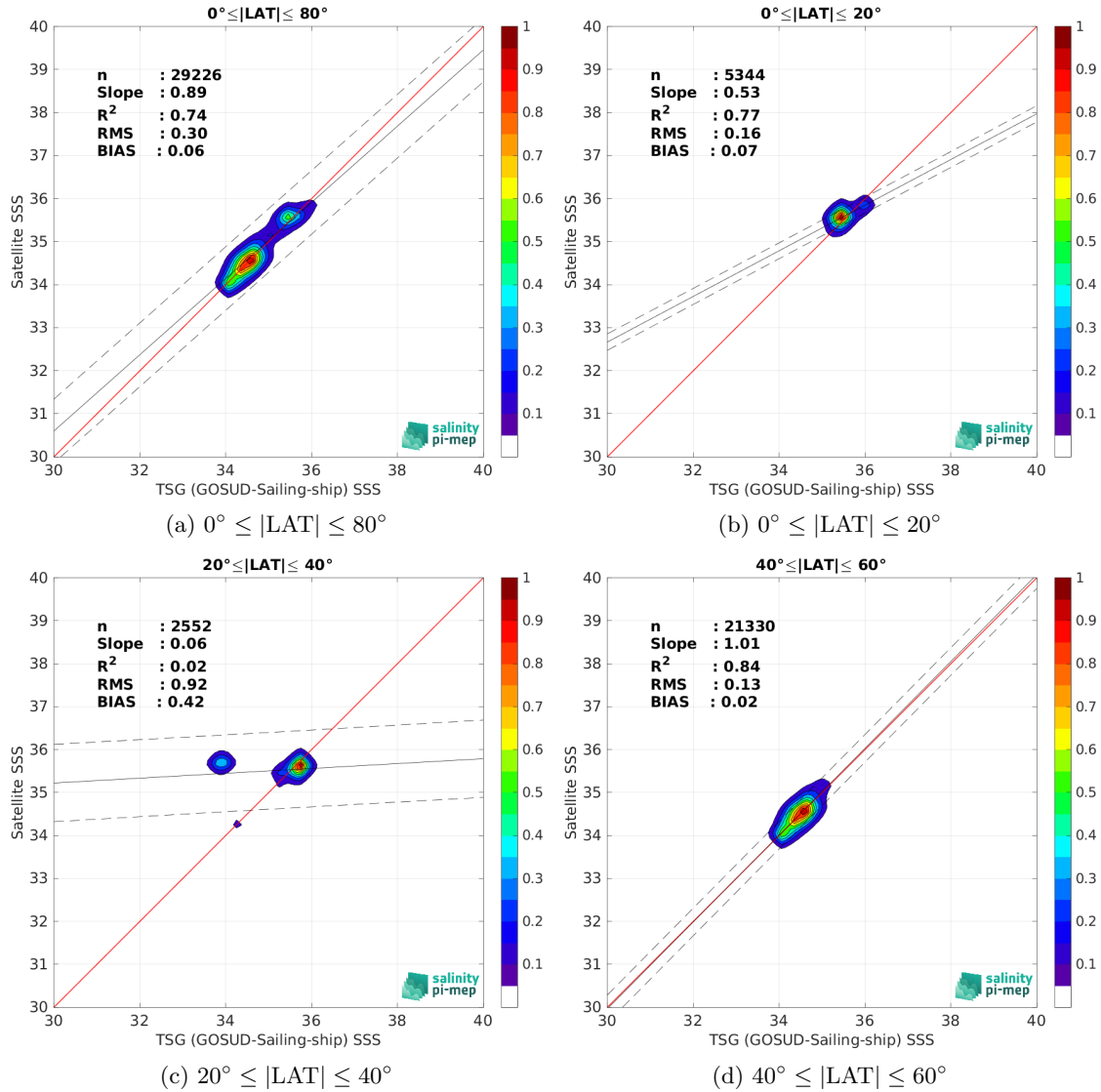
Figure 10: Contour maps of the concentration of SMAP SSS L4 OI v3 - Daily (ESR) SSS (y-axis) versus TSG (GOSUD-Sailing-ship) SSS (x-axis) at match-up pairs for different latitude bands. For each plot, the red line shows x=y . The black thin and dashed lines indicate a linear fit through the data cloud and the \pm 95\% confidence levels, respectively. The number match-up pairs n , the slope and R^2 coefficient of the linear fit, the root mean square (RMS) and the mean bias between satellite and in situ data are indicated for each latitude band in each plots.
