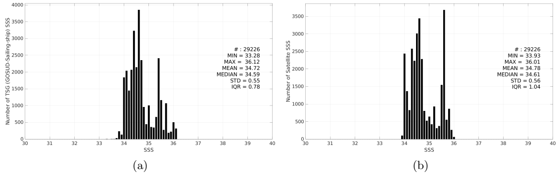
Figure 3: Histograms of SSS from TSG (GOSUD-Sailing-ship) (a) and SMAP SSS L4 OI v3 - Daily (ESR) (b) considering all match-up pairs per bins of 0.1 over the South Pacific Ocean Pi-MEP region and for the full satellite product period.
