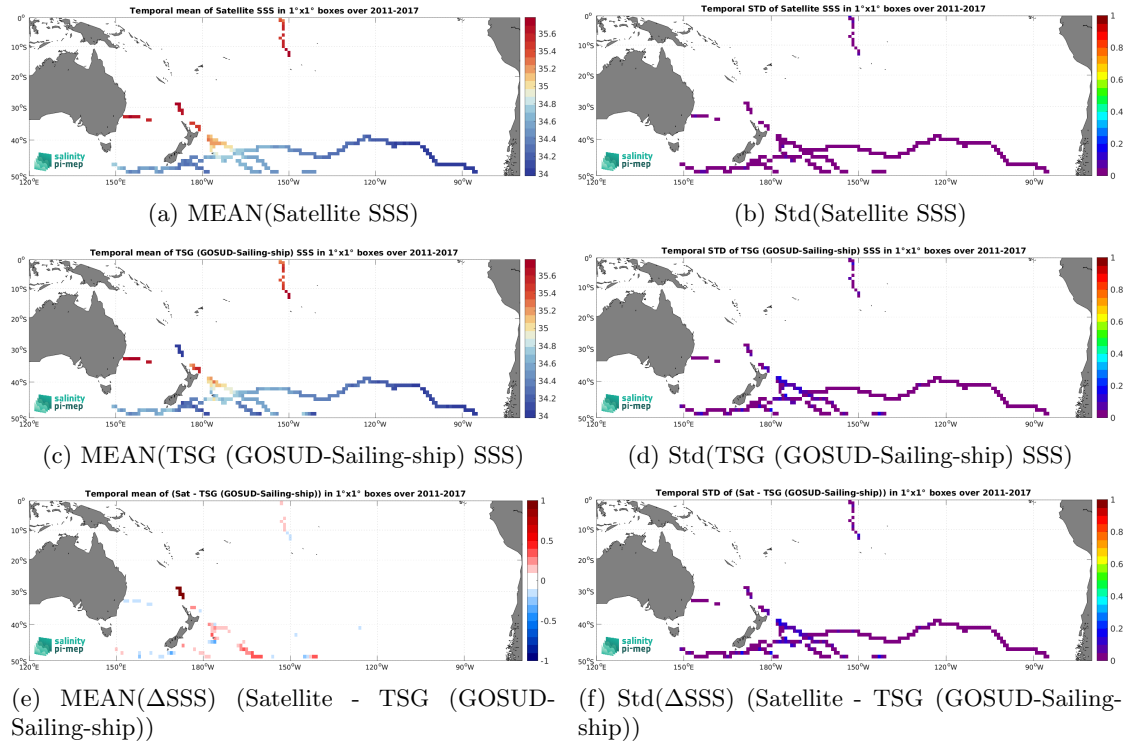
Figure 7: Temporal mean (left) and Std (right) of SSS from SMAP SSS L4 OI v3 - Daily (ESR) (top), TSG (GOSUD-Sailing-ship) (middle), and of \Delta SSS (Satellite - TSG (GOSUD-Sailing-ship)). Only match-up pairs are used to generate these maps.
