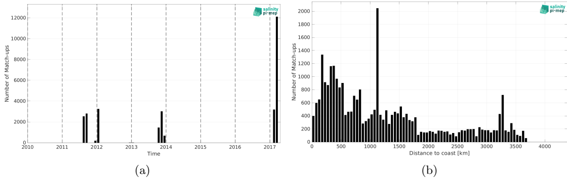
Figure 2: Number of match-ups between TSG (GOSUD-Sailing-ship) and SMAP SSS L4 OI v3 - Daily (ESR) SSS as a function of time (a) and as function of the distance to coast (b) over the South Pacific Ocean Pi-MEP region and for the full satellite product period.
