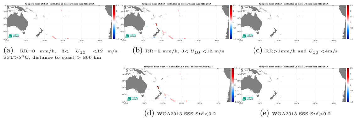
Figure 14: Temporal mean gridded over spatial boxes of size 1^\circ \times 1^\circ of \Delta SSS (SMAP SSS L4 OI v3 - Daily (ESR) - TSG (GOSUD-Sailing-ship)) for 5 different subdatasets corresponding to:RR=0 mm/h, 3 < U_{10} < 12 m/s, SST>5°C, distance to coast > 800 km (a), RR=0 mm/h, 3 < U_{10} < 12 m/s (b), RR>1mm/h and U_{10} < 4 m/s (c), WOA2013 SSS Std<0.2 (d), WOA2013 SSS Std>0.2 (e).
