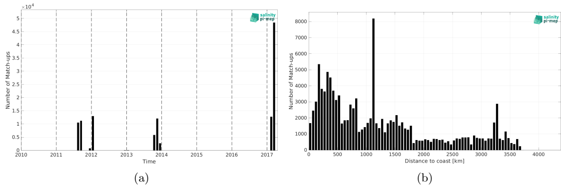
Figure 2: Number of match-ups between TSG (GOSUD-Sailing-ship) and SMAP SSS L4 OI v3 - Daily (ESR) SSS as a function of time (a) and as function of the distance to coast (b) over the South Pacific Ocean Pi-MEP region and for the full satellite product period.
