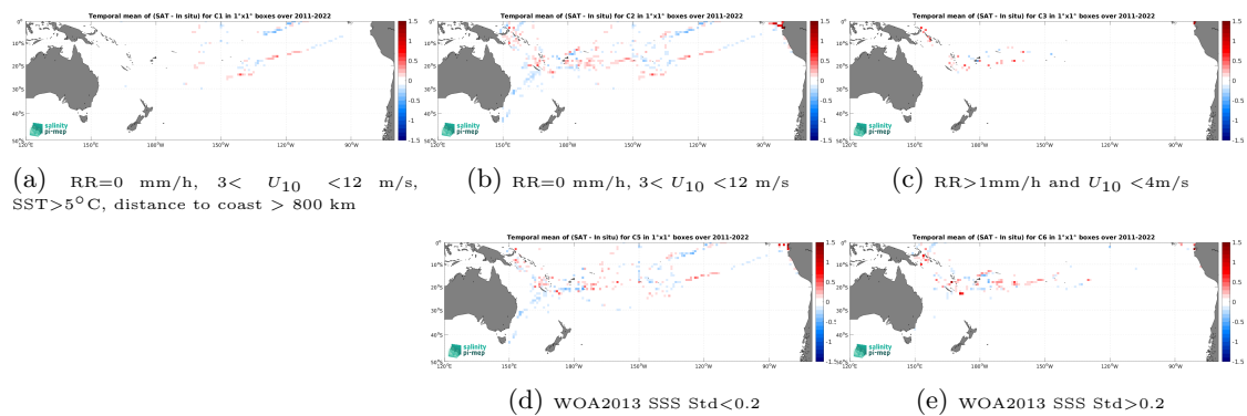
Figure 14: Temporal mean gridded over spatial boxes of size 1^\circ \times 1^\circ of \Delta\text{SSS} (SMAP SSS L4 OI v3 - Daily (ESR) - TSG (GOSUD-Research-vessel)) for 5 different subdatasets corresponding to:RR=0 mm/h, 3 < U_{10} < 12 m/s, SST >5^\circ\text{C} , distance to coast > 800 km (a), RR=0 mm/h, 3 < U_{10} < 12 m/s (b), RR >1 mm/h and U_{10} < 4 m/s (c), WOA2013 SSS Std <0.2 (d), WOA2013 SSS Std >0.2 (e).
