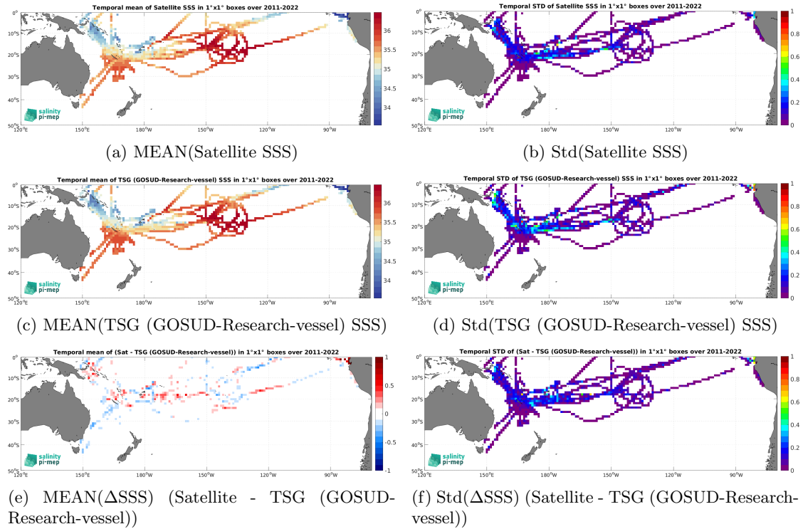
Figure 7: Temporal mean (left) and Std (right) of SSS from SMAP SSS L4 OI v3 - Daily (ESR) (top), TSG (GOSUD-Research-vessel) (middle), and of \Delta SSS (Satellite - TSG (GOSUD-Research-vessel)). Only match-up pairs are used to generate these maps.
