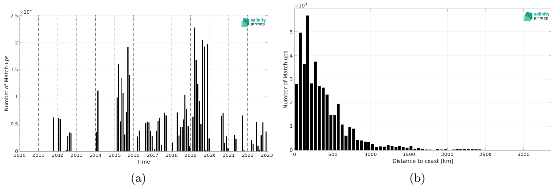
Figure 2: Number of match-ups between TSG (GOSUD-Research-vessel) and SMAP SSS L4 OI v3 - Daily (ESR) SSS as a function of time (a) and as function of the distance to coast (b) over the South Pacific Ocean Pi-MEP region and for the full satellite product period.
