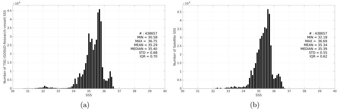
Figure 3: Histograms of SSS from TSG (GOSUD-Research-vessel) (a) and SMAP SSS L4 OI v3 - Daily (ESR) (b) considering all match-up pairs per bins of 0.1 over the South Pacific Ocean Pi-MEP region and for the full satellite product period.
