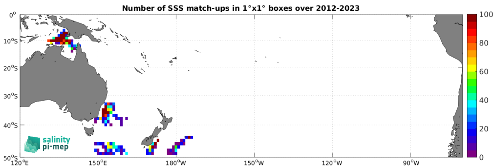
Figure 5: Number of SSS match-ups between Marine mammals SSS and the SMAP SSS L4 OI v3 - Daily (ESR) SSS product for the South Pacific Ocean Pi-MEP region over 1^\circ \times 1^\circ boxes and for the full satellite product period.
