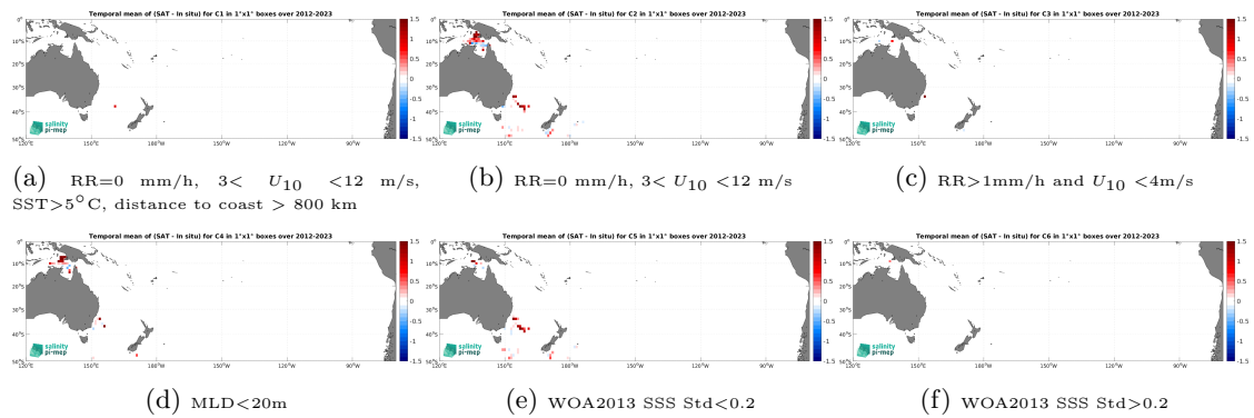
Figure 14: Temporal mean gridded over spatial boxes of size 1^\circ \times 1^\circ of \Delta SSS (SMAP SSS L4 OI v3 - Daily (ESR) - Marine mammals) for 6 different subdatasets corresponding to:RR=0 mm/h, 3 < U_{10} < 12 m/s, SST >5^\circ\text{C} , distance to coast > 800 km (a), RR=0 mm/h, 3 < U_{10} < 12 m/s (b), RR >1 mm/h and U_{10} < 4 m/s (c),MLD <20 m (d),WOA2013 SSS Std <0.2 (e),WOA2013 SSS Std >0.2 (f).
