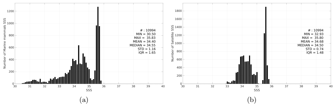
Figure 3: Histograms of SSS from Marine mammals (a) and SMAP SSS L4 OI v3 - Daily (ESR) (b) considering all match-up pairs per bins of 0.1 over the South Pacific Ocean Pi-MEP region and for the full satellite product period.
