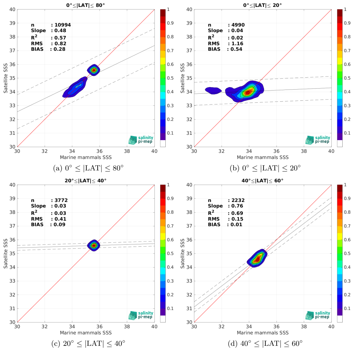
Figure 10: Contour maps of the concentration of SMAP SSS L4 OI v3 - Daily (ESR) SSS (y-axis) versus Marine mammals SSS (x-axis) at match-up pairs for different latitude bands. For each plot, the red line shows x=y . The black thin and dashed lines indicate a linear fit through the data cloud and the \pm 95\% confidence levels, respectively. The number match-up pairs n , the slope and R^2 coefficient of the linear fit, the root mean square (RMS) and the mean bias between satellite and in situ data are indicated for each latitude band in each plots.
