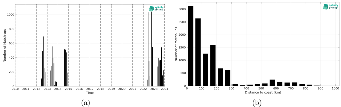
Figure 2: Number of match-ups between Marine mammals and SMAP SSS L4 OI v3 - Daily (ESR) SSS as a function of time (a) and as function of the distance to coast (b) over the South Pacific Ocean Pi-MEP region and for the full satellite product period.
