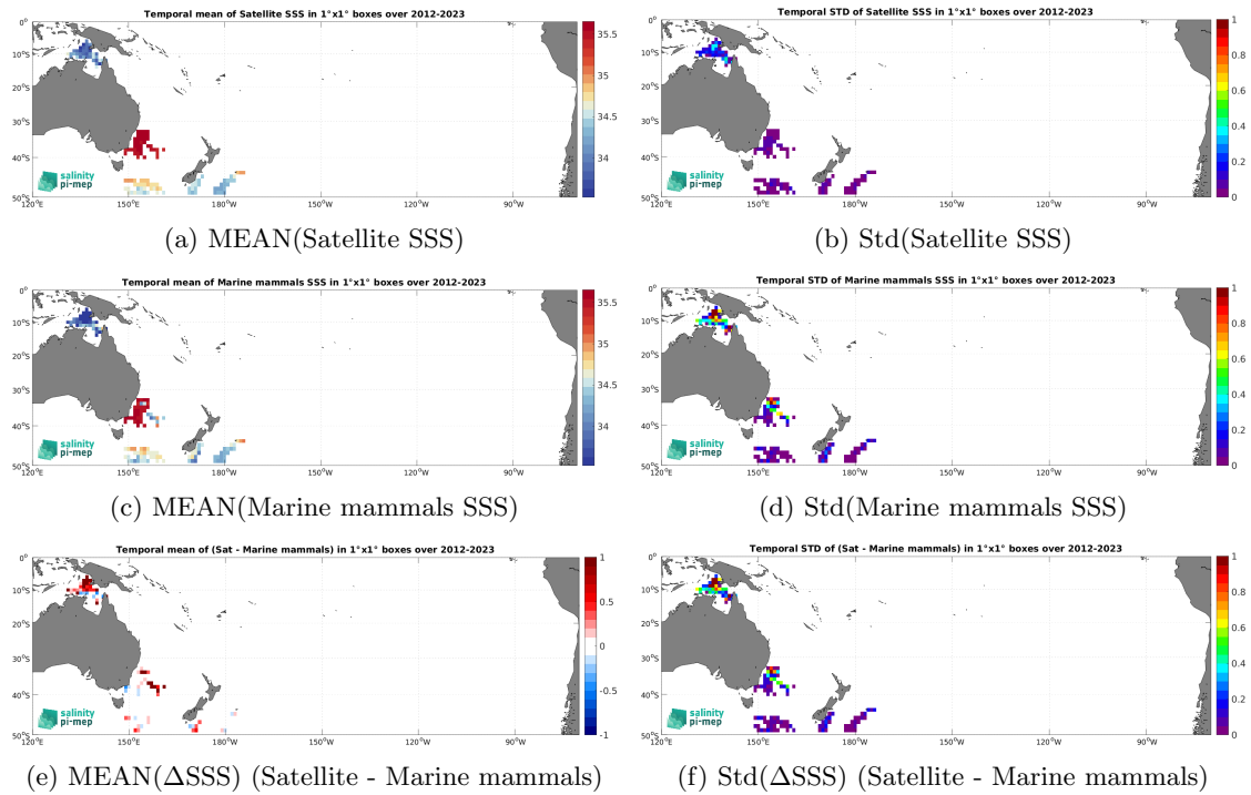
Figure 7: Temporal mean (left) and Std (right) of SSS from SMAP SSS L4 OI v3 - Daily (ESR) (top), Marine mammals (middle), and of \Delta SSS (Satellite - Marine mammals). Only match-up pairs are used to generate these maps.
