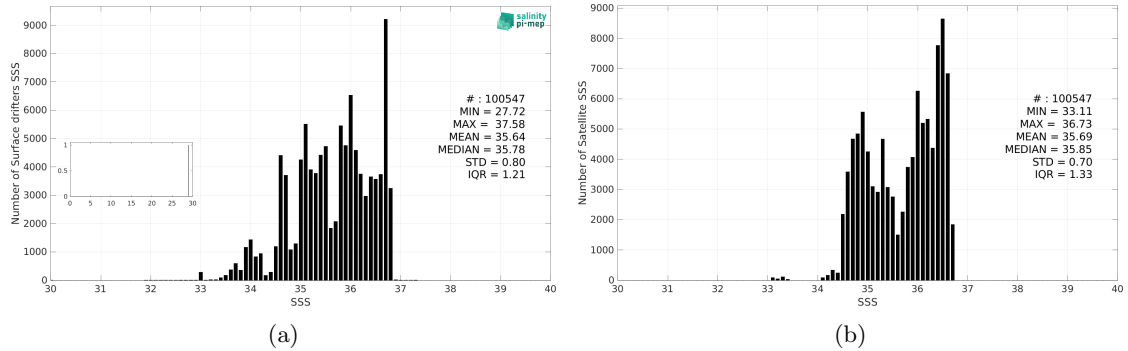
Figure 3: Histograms of SSS from Surface drifters (a) and SMAP SSS L4 OI v3 - Daily (ESR) (b) considering all match-up pairs per bins of 0.1 over the South Pacific Ocean Pi-MEP region and for the full satellite product period.
