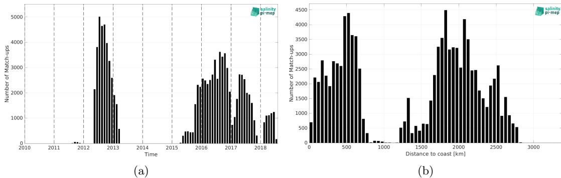
Figure 2: Number of match-ups between Surface drifters and SMAP SSS L4 OI v3 - Daily (ESR) SSS as a function of time (a) and as function of the distance to coast (b) over the South Pacific Ocean Pi-MEP region and for the full satellite product period.
