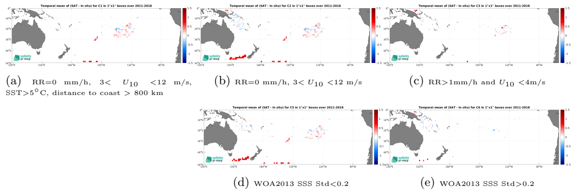
Figure 13: Temporal mean gridded over spatial boxes of size 1^\circ \times 1^\circ of \Delta SSS (SMAP SSS L4 OI v3 - Daily (ESR) - Surface drifters) for 5 different subdatasets corresponding to: RR=0 mm/h, 3 < U_{10} < 12 m/s, SST > 5^\circ C , distance to coast > 800 km (a), RR=0 mm/h, 3 < U_{10} < 12 m/s (b), RR > 1 mm/h and U_{10} < 4 m/s (c), WOA2013 SSS Std < 0.2 (d), WOA2013 SSS Std > 0.2 (e).
