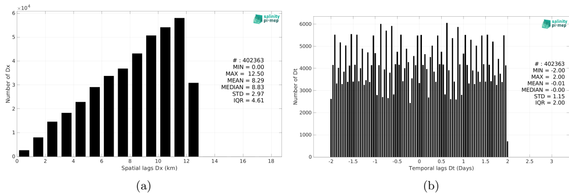
Figure 5: Histograms of the spatial (a) and temporal (b) lags between the location/time of the Surface drifters measurement and the date of the corresponding SMAP SSS L4 OI v3 - Daily (ESR) SSS pixel.
