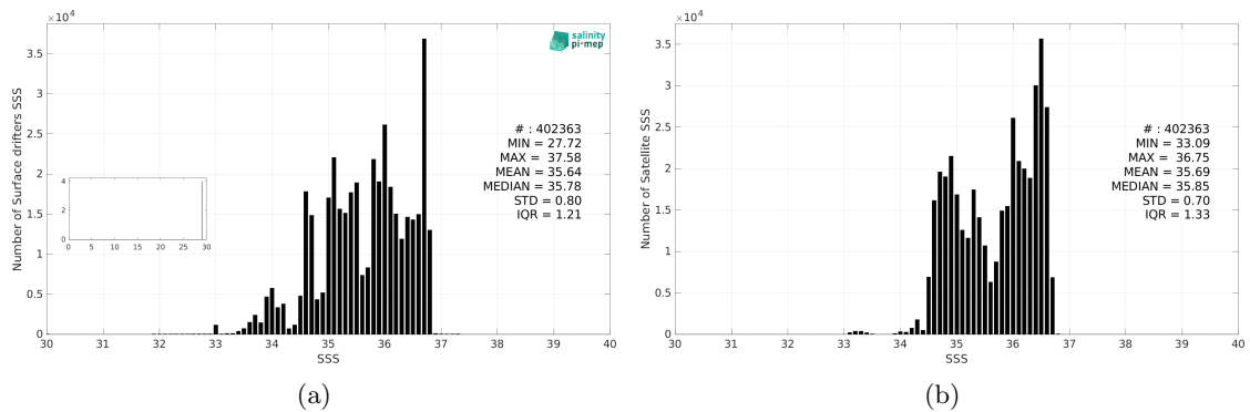
Figure 3: Histograms of SSS from Surface drifters (a) and SMAP SSS L4 OI v3 - Daily (ESR) (b) considering all match-up pairs per bins of 0.1 over the South Pacific Ocean Pi-MEP region and for the full satellite product period.
