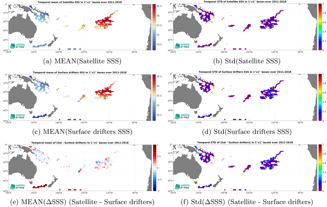
Figure 6: Temporal mean (left) and Std (right) of SSS from SMAP SSS L4 OI v3 - Daily (ESR) (top), Surface drifters (middle), and of \Delta SSS (Satellite - Surface drifters). Only match-up pairs are used to generate these maps.
