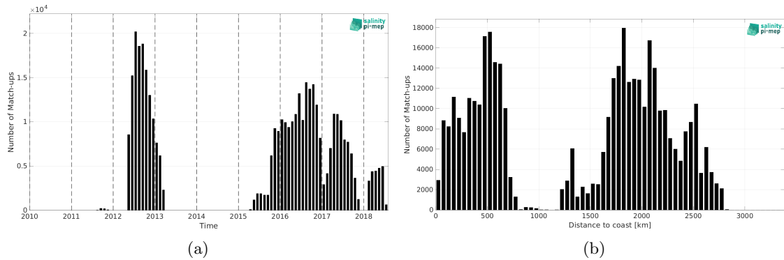
Figure 2: Number of match-ups between Surface drifters and SMAP SSS L4 OI v3 - Daily (ESR) SSS as a function of time (a) and as function of the distance to coast (b) over the South Pacific Ocean Pi-MEP region and for the full satellite product period.
