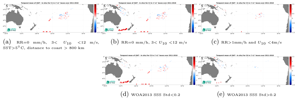
Figure 13: Temporal mean gridded over spatial boxes of size 1^\circ \times 1^\circ of \Delta\text{SSS} (SMAP SSS L4 OI v3 - Daily (ESR) - Surface drifters) for 5 different subdatasets corresponding to:RR=0 mm/h, 3 < U_{10} < 12 m/s, SST >5^\circ\text{C} , distance to coast > 800 km (a), RR=0 mm/h, 3 < U_{10} < 12 m/s (b), RR >1 mm/h and U_{10} < 4 m/s (c), WOA2013 SSS Std <0.2 (d), WOA2013 SSS Std >0.2 (e).
