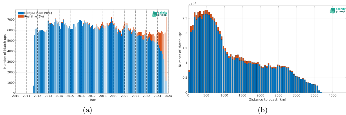
Figure 2: Number of match-ups between Argo and SMAP SSS L4 OI v3 - Daily (ESR) SSS as a function of time (a) and as function of the distance to coast (b) over the South Pacific Ocean Pi-MEP region and for the full satellite product period.
