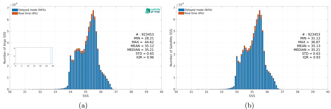
Figure 3: Histograms of SSS from Argo (a) and SMAP SSS L4 OI v3 - Daily (ESR) (b) considering all match-up pairs per bins of 0.1 over the South Pacific Ocean Pi-MEP region and for the full satellite product period.
