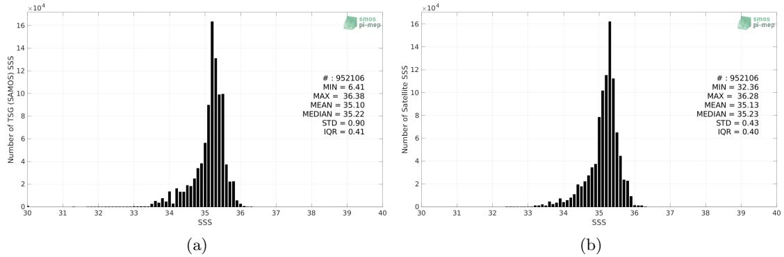
Figure 2: Histograms of SSS from TSG (SAMOS) (a) and SMAP SSS L4 OI v2 - 7 Days (ESR) (b) considering all match-up pairs per bins of 0.1 over the South Pacific Ocean Pi-MEP region and for the full satellite product period.
