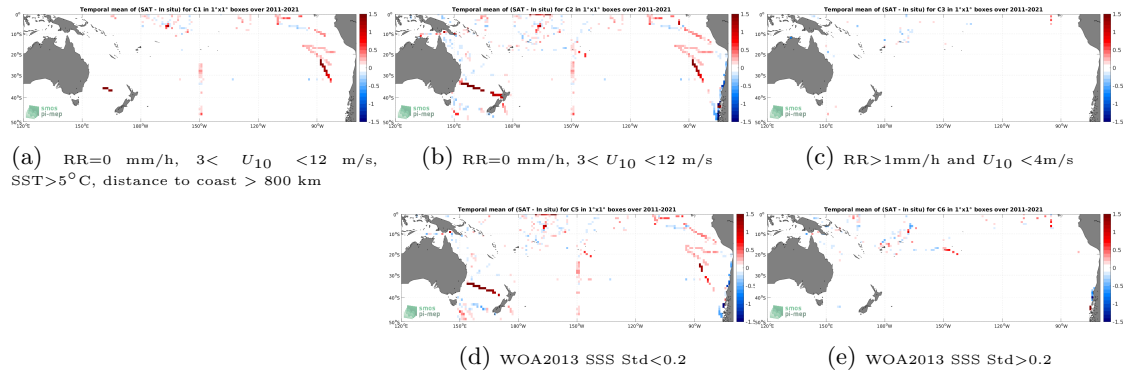
Figure 12: Temporal mean gridded over spatial boxes of size 1^\circ \times 1^\circ of \Delta SSS (SMAP SSS L4 OI v2 - 7 Days (ESR) - TSG (SAMOS)) for 5 different subdatasets corresponding to:RR=0 mm/h, 3 < U_{10} < 12 m/s, SST >5^\circ C, distance to coast > 800 km (a), RR=0 mm/h, 3 < U_{10} < 12 m/s (b), RR >1 mm/h and U_{10} < 4 m/s (c), WOA2013 SSS Std <0.2 (d), WOA2013 SSS Std >0.2 (e).
