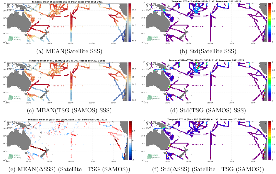
Figure 6: Temporal mean (left) and Std (right) of SSS from SMAP SSS L4 OI v2 - 7 Days (ESR) (top), TSG (SAMOS) (middle), and of \Delta SSS (Satellite - TSG (SAMOS)). Only match-up pairs are used to generate these maps.
