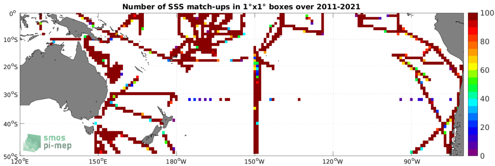
Figure 4: Number of SSS match-ups between TSG (SAMOS) SSS and the SMAP SSS L4 OI v2 - 7 Days (ESR) SSS product for the South Pacific Ocean Pi-MEP region over 1^\circ \times 1^\circ boxes and for the full satellite product period.
