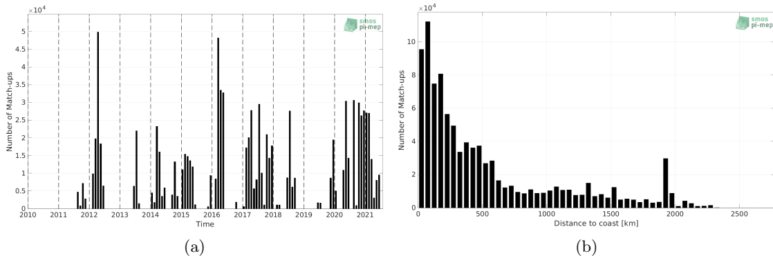
Figure 1: Number of match-ups between TSG (SAMOS) and SMAP SSS L4 OI v2 - 7 Days (ESR) SSS as a function of time (a) and as function of the distance to coast (b) over the South Pacific Ocean Pi-MEP region and for the full satellite product period.
