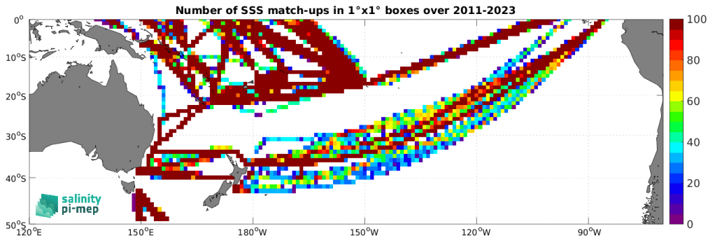
Figure 4: Number of SSS match-ups between TSG (LEGOS-DM) SSS and the SMAP SSS L4 OI v2 - 7 Days (ESR) SSS product for the South Pacific Ocean Pi-MEP region over 1^\circ \times 1^\circ boxes and for the full satellite product period.
