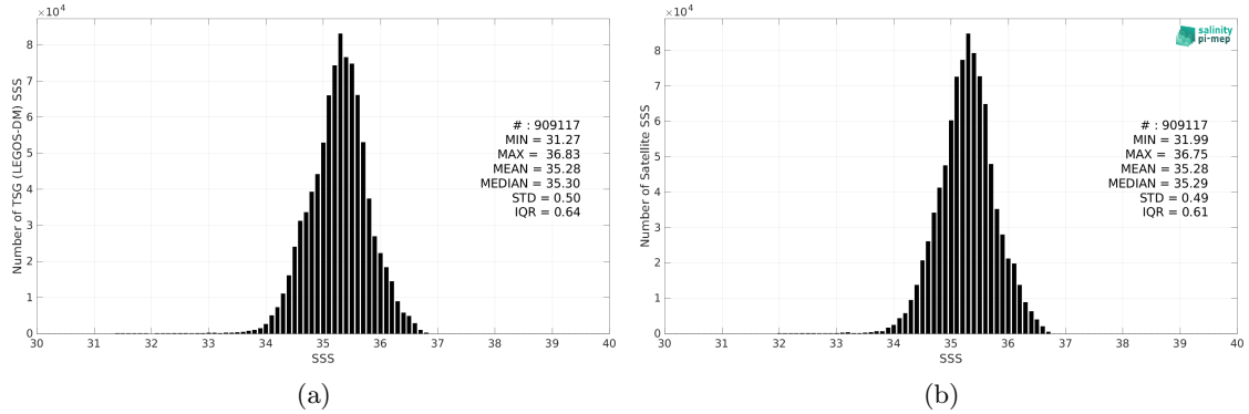
Figure 2: Histograms of SSS from TSG (LEGOS-DM) (a) and SMAP SSS L4 OI v2 - 7 Days (ESR) (b) considering all match-up pairs per bins of 0.1 over the South Pacific Ocean Pi-MEP region and for the full satellite product period.
