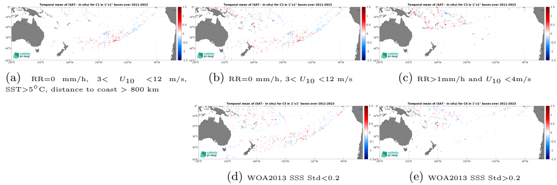
Figure 12: Temporal mean gridded over spatial boxes of size 1^\circ \times 1^\circ of \Delta SSS (SMAP SSS L4 OI v2 - 7 Days (ESR) - TSG (LEGOS-DM)) for 5 different subdatasets corresponding to:RR=0 mm/h, 3 < U_{10} < 12 m/s, SST >5^\circ\text{C} , distance to coast > 800 km (a), RR=0 mm/h, 3 < U_{10} < 12 m/s (b), RR >1 mm/h and U_{10} < 4 m/s (c), WOA2013 SSS Std <0.2 (d), WOA2013 SSS Std >0.2 (e).
