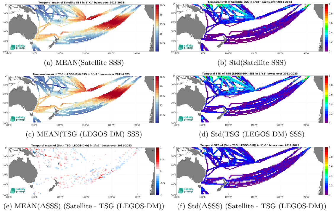
Figure 6: Temporal mean (left) and Std (right) of SSS from SMAP SSS L4 OI v2 - 7 Days (ESR) (top), TSG (LEGOS-DM) (middle), and of \Delta\text{SSS} (Satellite - TSG (LEGOS-DM)). Only match-up pairs are used to generate these maps.
