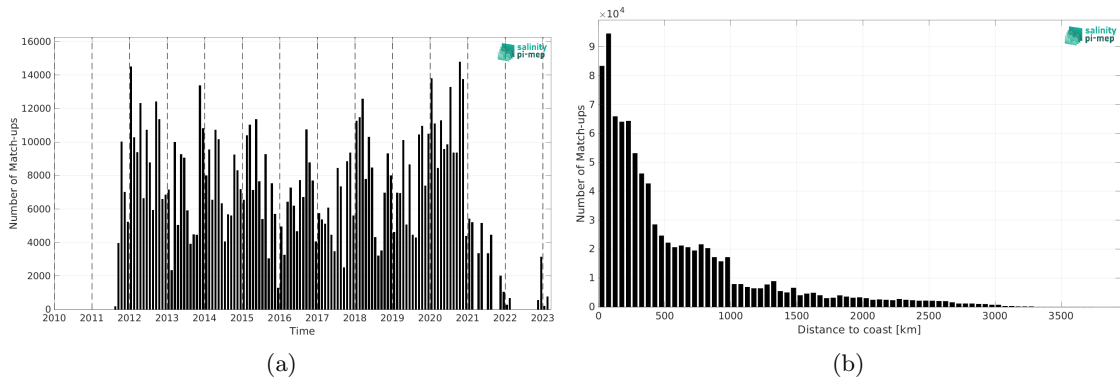
Figure 1: Number of match-ups between TSG (LEGOS-DM) and SMAP SSS L4 OI v2 - 7 Days (ESR) SSS as a function of time (a) and as function of the distance to coast (b) over the South Pacific Ocean Pi-MEP region and for the full satellite product period.
