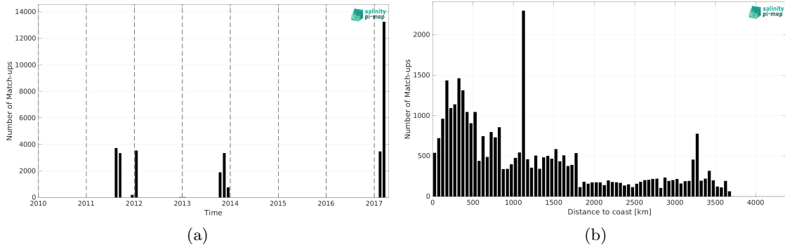
Figure 1: Number of match-ups between TSG (GOSUD-Sailing-ship) and SMAP SSS L4 OI v2 - 7 Days (ESR) SSS as a function of time (a) and as function of the distance to coast (b) over the South Pacific Ocean Pi-MEP region and for the full satellite product period.
