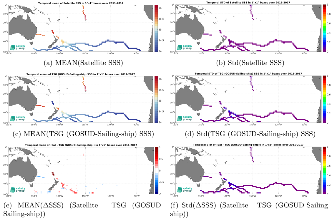
Figure 6: Temporal mean (left) and Std (right) of SSS from SMAP SSS L4 OI v2 - 7 Days (ESR) (top), TSG (GOSUD-Sailing-ship) (middle), and of \Delta SSS (Satellite - TSG (GOSUD-Sailing-ship)). Only match-up pairs are used to generate these maps.
