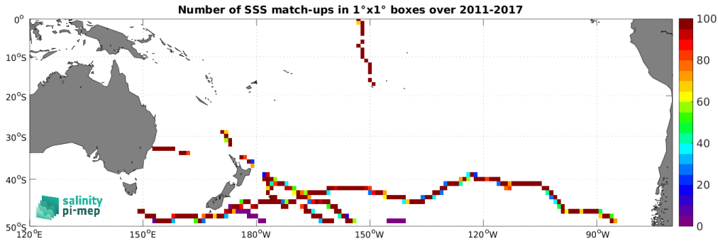
Figure 4: Number of SSS match-ups between TSG (GOSUD-Sailing-ship) SSS and the SMAP SSS L4 OI v2 - 7 Days (ESR) SSS product for the South Pacific Ocean Pi-MEP region over 1^\circ \times 1^\circ boxes and for the full satellite product period.
