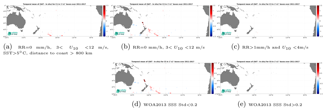
Figure 12: Temporal mean gridded over spatial boxes of size 1^\circ \times 1^\circ of \Delta SSS (SMAP SSS L4 OI v2 - 7 Days (ESR) - TSG (GOSUD-Sailing-ship)) for 5 different subdatasets corresponding to:RR=0 mm/h, 3 < U_{10} < 12 m/s, SST>5°C, distance to coast > 800 km (a), RR=0 mm/h, 3 < U_{10} < 12 m/s (b), RR>1mm/h and U_{10} < 4 m/s (c), WOA2013 SSS Std<0.2 (d), WOA2013 SSS Std>0.2 (e).
