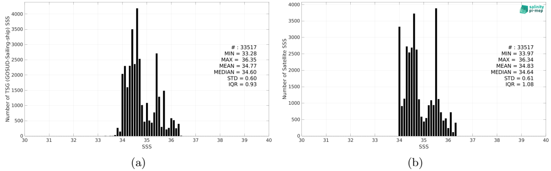
Figure 2: Histograms of SSS from TSG (GOSUD-Sailing-ship) (a) and SMAP SSS L4 OI v2 - 7 Days (ESR) (b) considering all match-up pairs per bins of 0.1 over the South Pacific Ocean Pi-MEP region and for the full satellite product period.
