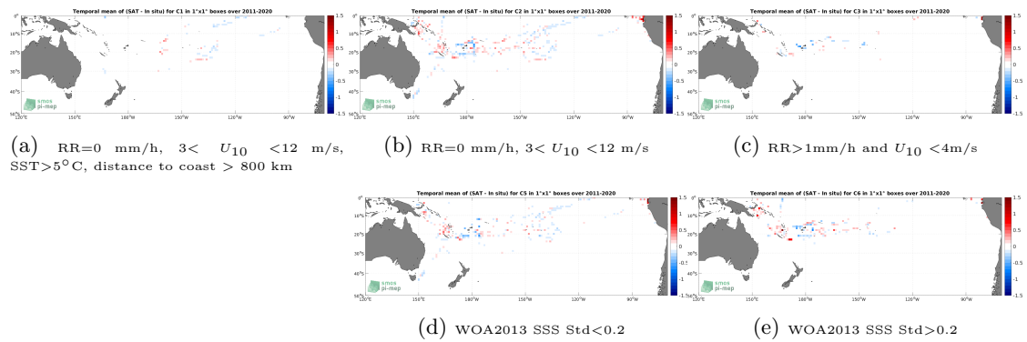
Figure 12: Temporal mean gridded over spatial boxes of size 1^\circ \times 1^\circ of \Delta SSS (SMAP SSS L4 OI v2 - 7 Days (ESR) - TSG (GOSUD-Research-vessel)) for 5 different subdatasets corresponding to:RR=0 mm/h, 3 < U_{10} < 12 m/s, SST >5^\circ C, distance to coast > 800 km (a), RR=0 mm/h, 3 < U_{10} < 12 m/s (b), RR >1 mm/h and U_{10} < 4 m/s (c), WOA2013 SSS Std <0.2 (d), WOA2013 SSS Std >0.2 (e).
