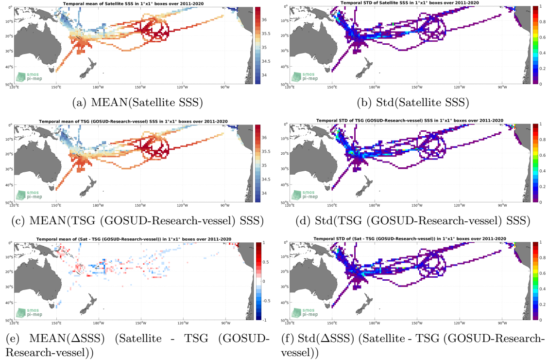
Figure 6: Temporal mean (left) and Std (right) of SSS from SMAP SSS L4 OI v2 - 7 Days (ESR) (top), TSG (GOSUD-Research-vessel) (middle), and of \Delta SSS (Satellite - TSG (GOSUD-Research-vessel)). Only match-up pairs are used to generate these maps.
