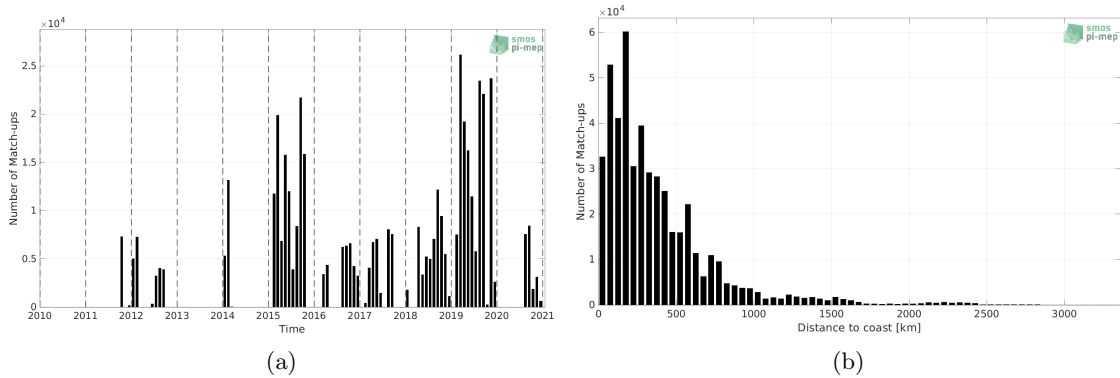
Figure 1: Number of match-ups between TSG (GOSUD-Research-vessel) and SMAP SSS L4 OI v2 - 7 Days (ESR) SSS as a function of time (a) and as function of the distance to coast (b) over the South Pacific Ocean Pi-MEP region and for the full satellite product period.
