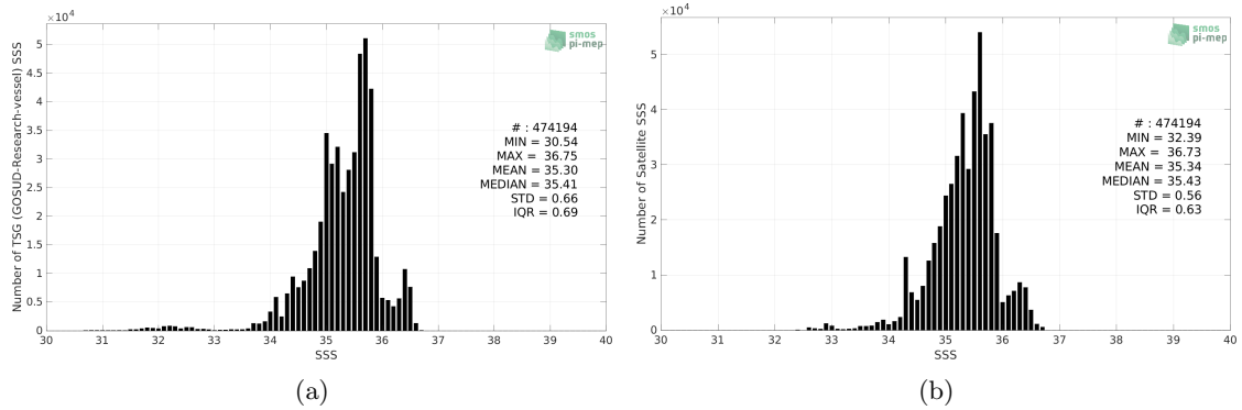
Figure 2: Histograms of SSS from TSG (GOSUD-Research-vessel) (a) and SMAP SSS L4 OI v2 - 7 Days (ESR) (b) considering all match-up pairs per bins of 0.1 over the South Pacific Ocean Pi-MEP region and for the full satellite product period.
