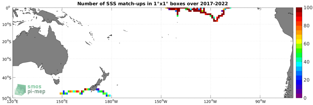
Figure 4: Number of SSS match-ups between Saildrone SSS and the SMAP SSS L4 OI v2 - 7 Days (ESR) SSS product for the South Pacific Ocean Pi-MEP region over 1^\circ \times 1^\circ boxes and for the full satellite product period.
