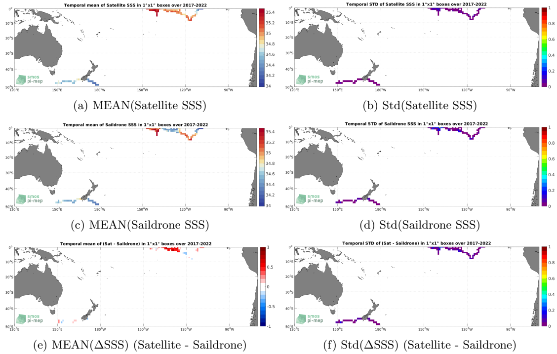
Figure 6: Temporal mean (left) and Std (right) of SSS from SMAP SSS L4 OI v2 - 7 Days (ESR) (top), Saildrone (middle), and of \Delta SSS (Satellite - Saildrone). Only match-up pairs are used to generate these maps.
