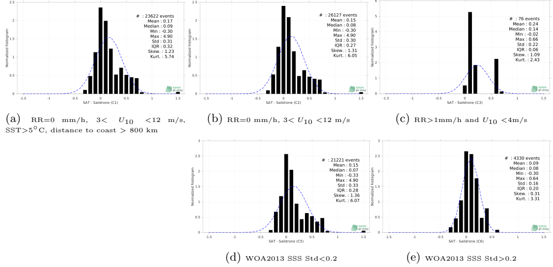
Figure 13: Normalized histogram of \Delta SSS (SMAP SSS L4 OI v2 - 7 Days (ESR) - Saildrone) for 5 different subdatasets corresponding to: RR=0 mm/h, 3 < U_{10} < 12 m/s, SST > 5°C, distance to coast > 800 km (a), RR=0 mm/h, 3 < U_{10} < 12 m/s (b), RR > 1mm/h and U_{10} < 4 m/s (c), WOA2013 SSS Std < 0.2 (d), WOA2013 SSS Std > 0.2 (e).
