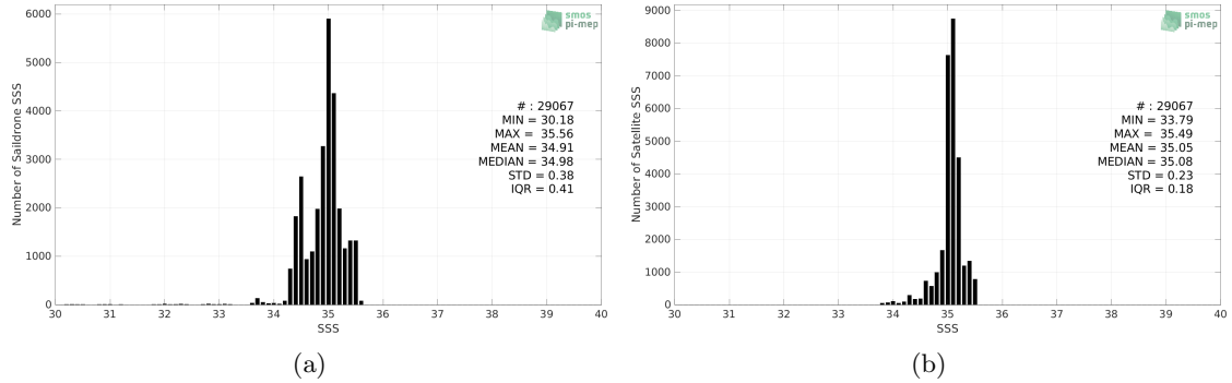
Figure 2: Histograms of SSS from Saildrone (a) and SMAP SSS L4 OI v2 - 7 Days (ESR) (b) considering all match-up pairs per bins of 0.1 over the South Pacific Ocean Pi-MEP region and for the full satellite product period.
