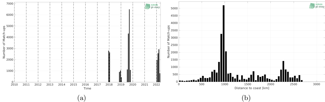
Figure 1: Number of match-ups between Saildrone and SMAP SSS L4 OI v2 - 7 Days (ESR) SSS as a function of time (a) and as function of the distance to coast (b) over the South Pacific Ocean Pi-MEP region and for the full satellite product period.
