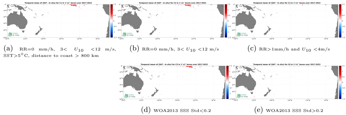
Figure 12: Temporal mean gridded over spatial boxes of size 1^\circ \times 1^\circ of \Delta SSS (SMAP SSS L4 OI v2 - 7 Days (ESR) - Saildrone) for 5 different subdatasets corresponding to:RR=0 mm/h, 3 < U_{10} < 12 m/s, SST >5^\circ C, distance to coast > 800 km (a), RR=0 mm/h, 3 < U_{10} < 12 m/s (b), RR >1 mm/h and U_{10} < 4 m/s (c), WOA2013 SSS Std <0.2 (d), WOA2013 SSS Std >0.2 (e).
