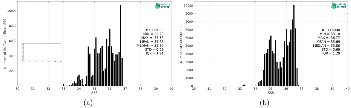
Figure 2: Histograms of SSS from Surface drifters (a) and SMAP SSS L4 OI v2 - 7 Days (ESR) (b) considering all match-up pairs per bins of 0.1 over the South Pacific Ocean Pi-MEP region and for the full satellite product period.
