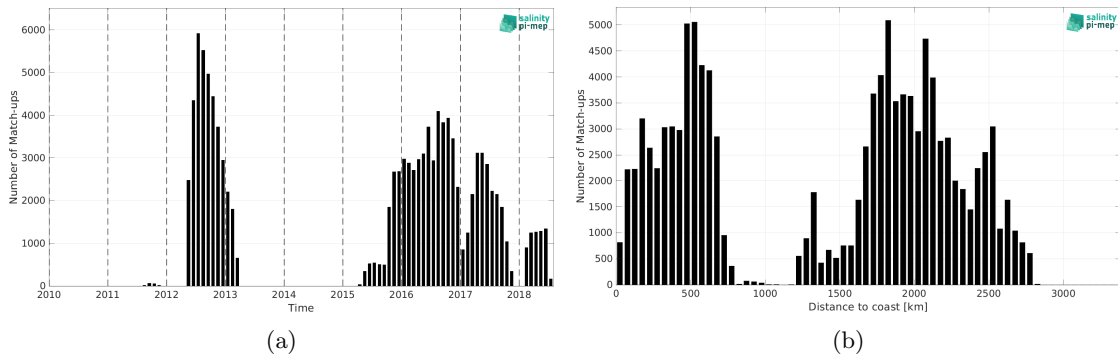
Figure 1: Number of match-ups between Surface drifters and SMAP SSS L4 OI v2 - 7 Days (ESR) SSS as a function of time (a) and as function of the distance to coast (b) over the South Pacific Ocean Pi-MEP region and for the full satellite product period.
