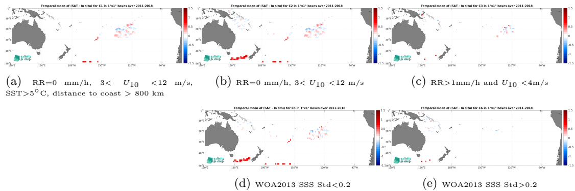
Figure 11: Temporal mean gridded over spatial boxes of size 1^\circ \times 1^\circ of \Delta SSS (SMAP SSS L4 OI v2 - 7 Days (ESR) - Surface drifters) for 5 different subdatasets corresponding to:RR=0 mm/h, 3 < U_{10} < 12 m/s, SST >5^\circ\text{C} , distance to coast > 800 km (a), RR=0 mm/h, 3 < U_{10} < 12 m/s (b), RR >1 mm/h and U_{10} < 4 m/s (c), WOA2013 SSS Std <0.2 (d), WOA2013 SSS Std >0.2 (e).
