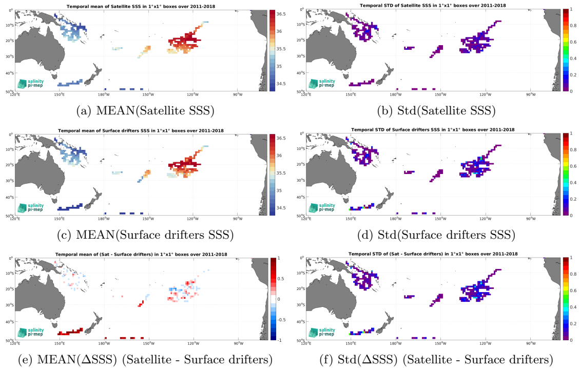
Figure 5: Temporal mean (left) and Std (right) of SSS from SMAP SSS L4 OI v2 - 7 Days (ESR) (top), Surface drifters (middle), and of \Delta SSS (Satellite - Surface drifters). Only match-up pairs are used to generate these maps.
