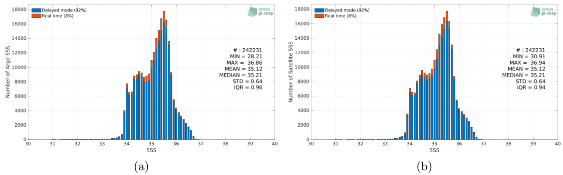
Figure 2: Histograms of SSS from Argo (a) and SMAP SSS L4 OI v2 - 7 Days (ESR) (b) considering all match-up pairs per bins of 0.1 over the South Pacific Ocean Pi-MEP region and for the full satellite product period.
