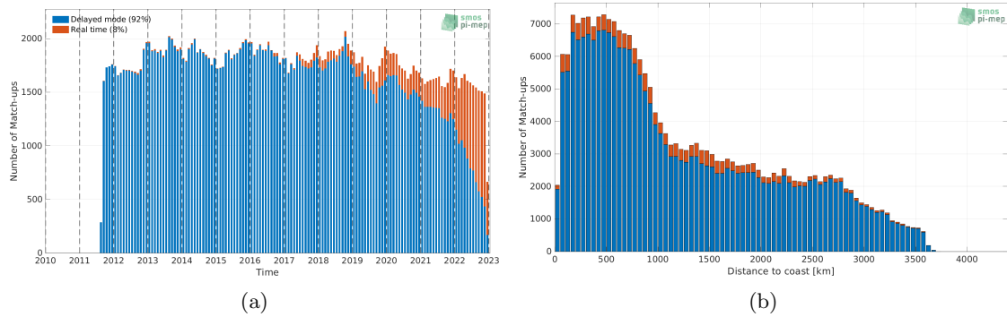
Figure 1: Number of match-ups between Argo and SMAP SSS L4 OI v2 - 7 Days (ESR) SSS as a function of time (a) and as function of the distance to coast (b) over the South Pacific Ocean Pi-MEP region and for the full satellite product period.
