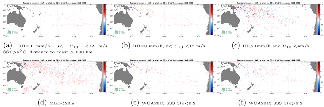
Figure 12: Temporal mean gridded over spatial boxes of size 1^\circ \times 1^\circ of \Delta SSS (SMAP SSS L4 OI v2 - 7 Days (ESR) - Argo) for 6 different subdatasets corresponding to:RR=0 mm/h, 3 < U_{10} < 12 m/s, SST >5^\circ\text{C} , distance to coast > 800 km (a), RR=0 mm/h, 3 < U_{10} < 12 m/s (b), RR >1 mm/h and U_{10} < 4 m/s (c),MLD <20 m (d),WOA2013 SSS Std <0.2 (e),WOA2013 SSS Std >0.2 (f).
