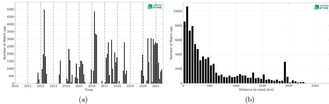
Figure 1: Number of match-ups between TSG (SAMOS) and SMAP SSS L4 OI v2 - Monthly (IPRC) SSS as a function of time (a) and as function of the distance to coast (b) over the South Pacific Ocean Pi-MEP region and for the full satellite product period.
