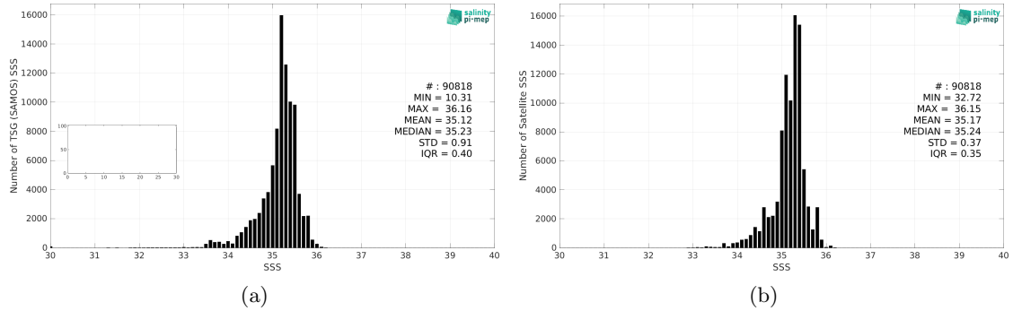
Figure 2: Histograms of SSS from TSG (SAMOS) (a) and SMAP SSS L4 OI v2 - Monthly (IPRC) (b) considering all match-up pairs per bins of 0.1 over the South Pacific Ocean Pi-MEP region and for the full satellite product period.
