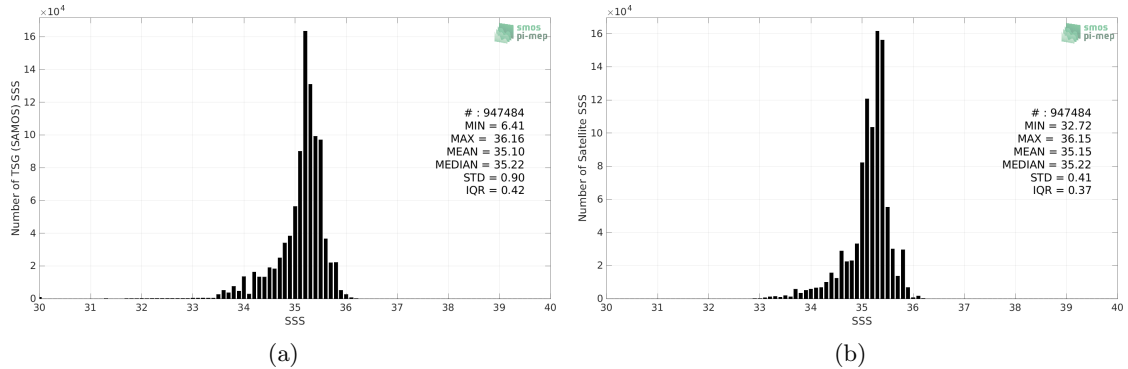
Figure 2: Histograms of SSS from TSG (SAMOS) (a) and SMAP SSS L4 OI v2 - Monthly (IPRC) (b) considering all match-up pairs per bins of 0.1 over the South Pacific Ocean Pi-MEP region and for the full satellite product period.
