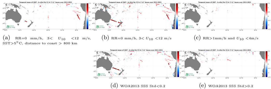
Figure 12: Temporal mean gridded over spatial boxes of size 1^\circ \times 1^\circ of \Delta SSS (SMAP SSS L4 OI v2 - Monthly (IPRC) - TSG (SAMOS)) for 5 different subdatasets corresponding to:RR=0 mm/h, 3 < U_{10} < 12 m/s, SST >5^\circ C, distance to coast > 800 km (a), RR=0 mm/h, 3 < U_{10} < 12 m/s (b), RR >1 mm/h and U_{10} < 4 m/s (c), WOA2013 SSS Std <0.2 (d), WOA2013 SSS Std >0.2 (e).
