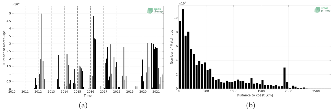
Figure 1: Number of match-ups between TSG (SAMOS) and SMAP SSS L4 OI v2 - Monthly (IPRC) SSS as a function of time (a) and as function of the distance to coast (b) over the South Pacific Ocean Pi-MEP region and for the full satellite product period.
