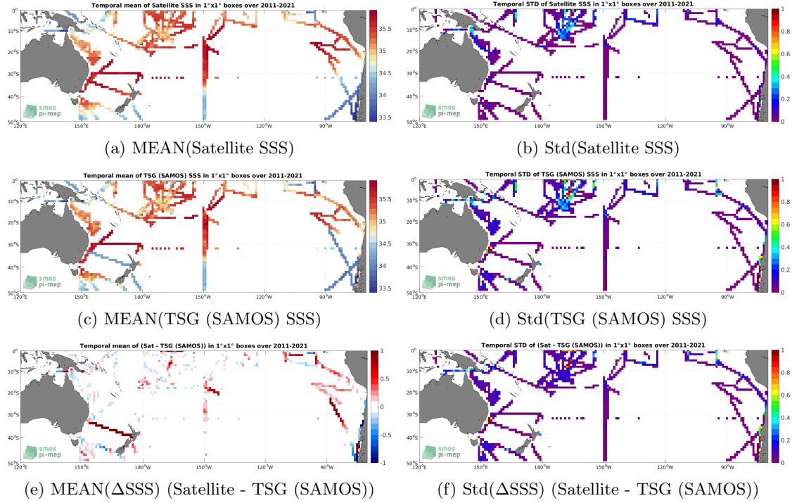
Figure 6: Temporal mean (left) and Std (right) of SSS from SMAP SSS L4 OI v2 - Monthly (IPRC) (top), TSG (SAMOS) (middle), and of \Delta SSS (Satellite - TSG (SAMOS)). Only match-up pairs are used to generate these maps.
