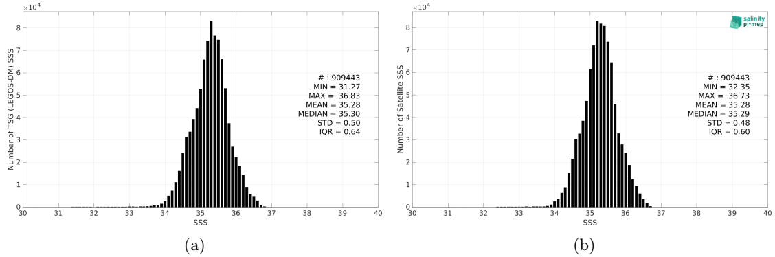
Figure 2: Histograms of SSS from TSG (LEGOS-DM) (a) and SMAP SSS L4 OI v2 - Monthly (IPRC) (b) considering all match-up pairs per bins of 0.1 over the South Pacific Ocean Pi-MEP region and for the full satellite product period.
