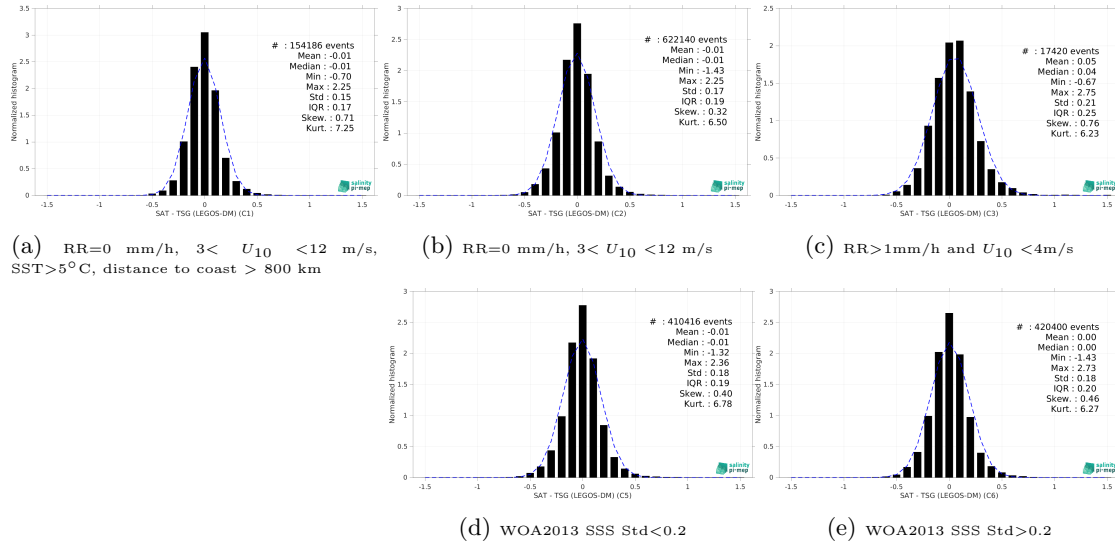
Figure 13: Normalized histogram of \Delta\text{SSS} (SMAP SSS L4 OI v2 - Monthly (IPRC) - TSG (LEGOS-DM)) for 5 different subdatasets corresponding to: RR=0 mm/h, 3 < U_{10} < 12 m/s, SST>5°C, distance to coast > 800 km (a), RR=0 mm/h, 3 < U_{10} < 12 m/s (b), RR>1mm/h and U_{10} < 4 m/s (c), WOA2013 SSS Std<0.2 (d), WOA2013 SSS Std>0.2 (e).
