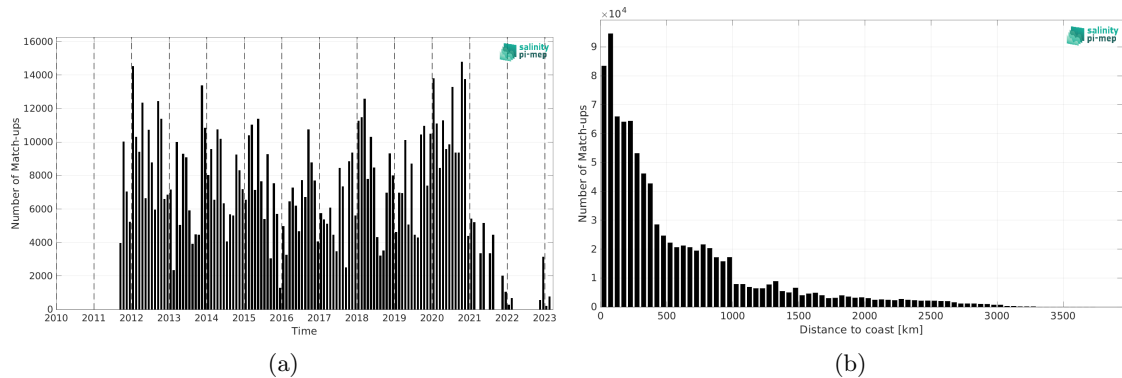
Figure 1: Number of match-ups between TSG (LEGOS-DM) and SMAP SSS L4 OI v2 - Monthly (IPRC) SSS as a function of time (a) and as function of the distance to coast (b) over the South Pacific Ocean Pi-MEP region and for the full satellite product period.
