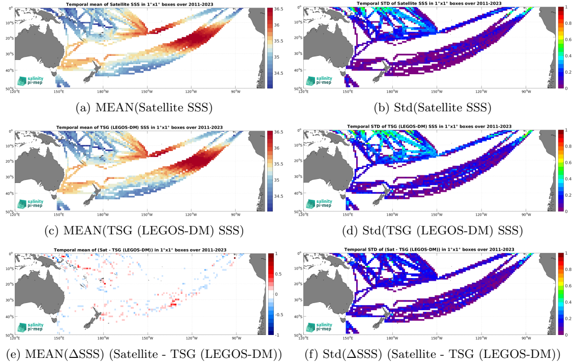
Figure 6: Temporal mean (left) and Std (right) of SSS from SMAP SSS L4 OI v2 - Monthly (IPRC) (top), TSG (LEGOS-DM) (middle), and of \Delta\text{SSS} (Satellite - TSG (LEGOS-DM)). Only match-up pairs are used to generate these maps.
