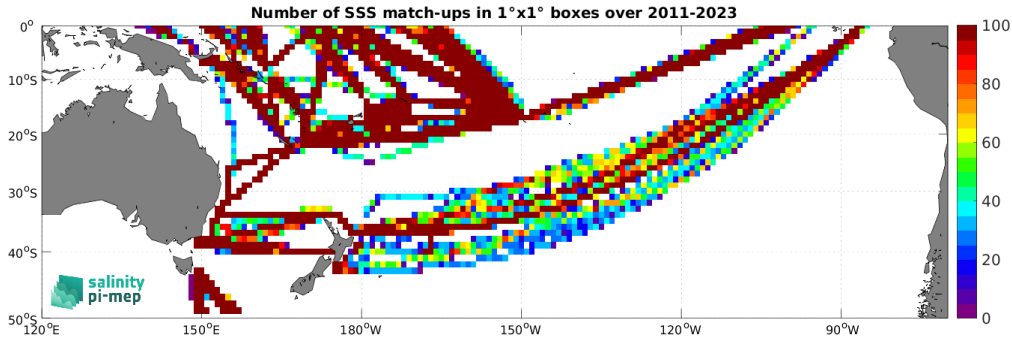
Figure 4: Number of SSS match-ups between TSG (LEGOS-DM) SSS and the SMAP SSS L4 OI v2 - Monthly (IPRC) SSS product for the South Pacific Ocean Pi-MEP region over 1^\circ \times 1^\circ boxes and for the full satellite product period.
