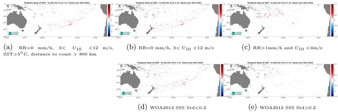
Figure 12: Temporal mean gridded over spatial boxes of size 1^\circ \times 1^\circ of \Delta SSS (SMAP SSS L4 OI v2 - Monthly (IPRC) - TSG (LEGOS-DM)) for 5 different subdatasets corresponding to:RR=0 mm/h, 3 < U_{10} < 12 m/s, SST >5^\circ\text{C} , distance to coast > 800 km (a), RR=0 mm/h, 3 < U_{10} < 12 m/s (b), RR >1 mm/h and U_{10} < 4 m/s (c), WOA2013 SSS Std <0.2 (d), WOA2013 SSS Std >0.2 (e).
