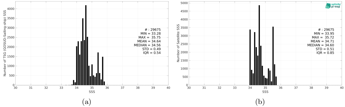
Figure 2: Histograms of SSS from TSG (GOSUD-Sailing-ship) (a) and SMAP SSS L4 OI v2 - Monthly (IPRC) (b) considering all match-up pairs per bins of 0.1 over the South Pacific Ocean Pi-MEP region and for the full satellite product period.
