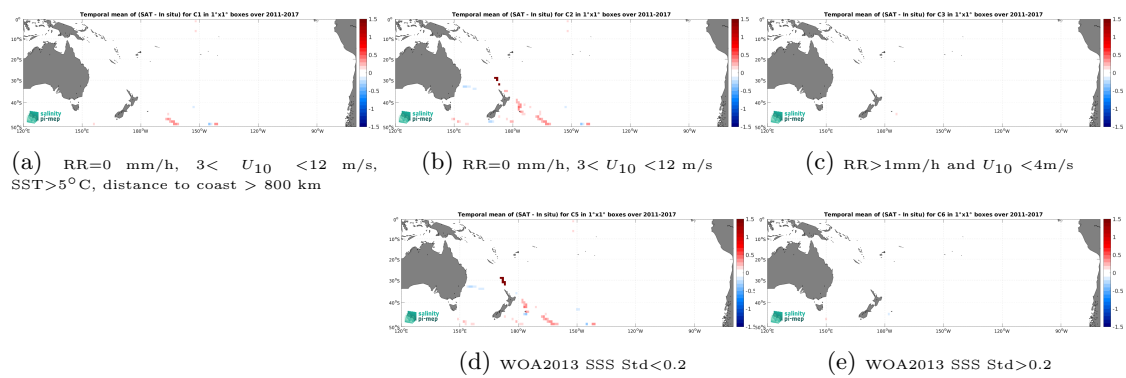
Figure 12: Temporal mean gridded over spatial boxes of size 1^\circ \times 1^\circ of \Delta SSS (SMAP SSS L4 OI v2 - Monthly (IPRC) - TSG (GOSUD-Sailing-ship)) for 5 different subdatasets corresponding to:RR=0 mm/h, 3 < U_{10} < 12 m/s, SST >5^\circ\text{C} , distance to coast > 800 km (a), RR=0 mm/h, 3 < U_{10} < 12 m/s (b), RR >1 mm/h and U_{10} < 4 m/s (c), WOA2013 SSS Std <0.2 (d), WOA2013 SSS Std >0.2 (e).
