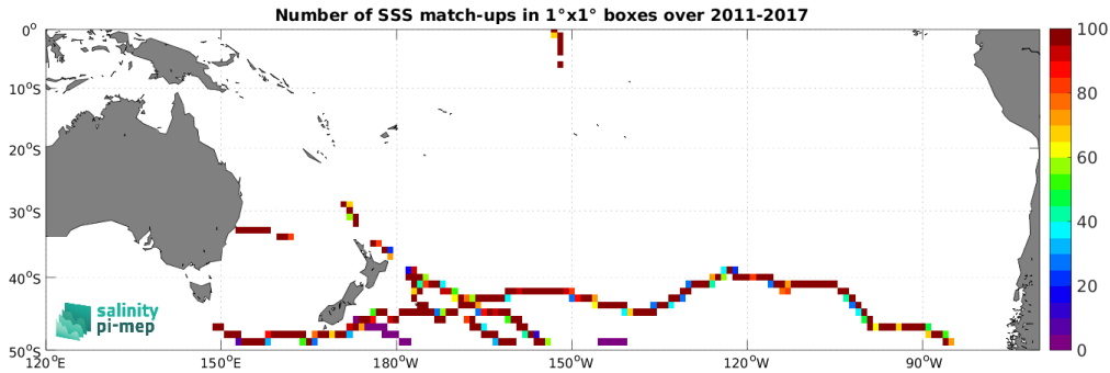
Figure 4: Number of SSS match-ups between TSG (GOSUD-Sailing-ship) SSS and the SMAP SSS L4 OI v2 - Monthly (IPRC) SSS product for the South Pacific Ocean Pi-MEP region over 1^\circ \times 1^\circ boxes and for the full satellite product period.
