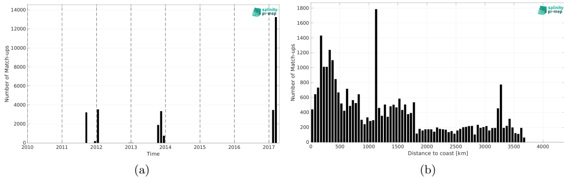
Figure 1: Number of match-ups between TSG (GOSUD-Sailing-ship) and SMAP SSS L4 OI v2 - Monthly (IPRC) SSS as a function of time (a) and as function of the distance to coast (b) over the South Pacific Ocean Pi-MEP region and for the full satellite product period.
