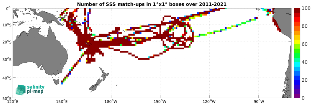
Figure 4: Number of SSS match-ups between TSG (GOSUD-Research-vessel) SSS and the SMAP SSS L4 OI v2 - Monthly (IPRC) SSS product for the South Pacific Ocean Pi-MEP region over 1^\circ \times 1^\circ boxes and for the full satellite product period.
