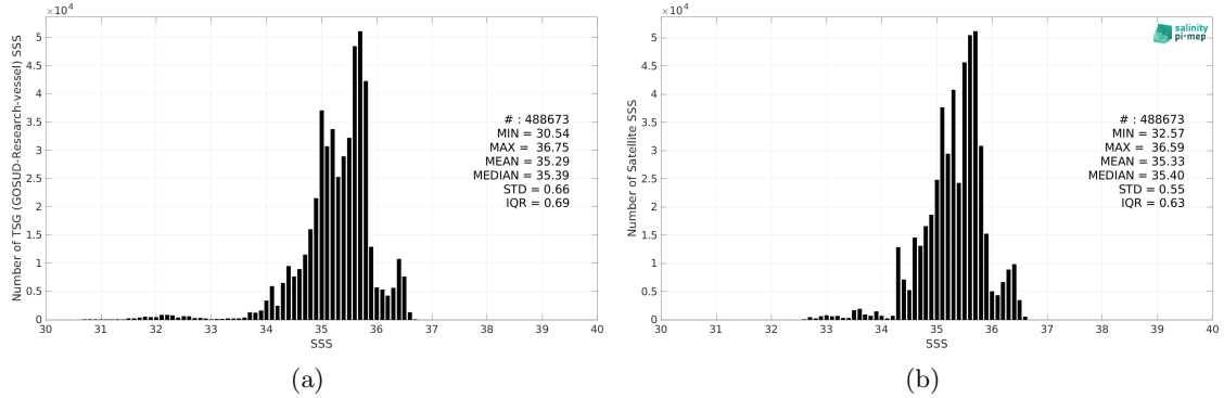
Figure 2: Histograms of SSS from TSG (GOSUD-Research-vessel) (a) and SMAP SSS L4 OI v2 - Monthly (IPRC) (b) considering all match-up pairs per bins of 0.1 over the South Pacific Ocean Pi-MEP region and for the full satellite product period.
