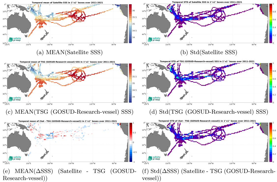
Figure 6: Temporal mean (left) and Std (right) of SSS from SMAP SSS L4 OI v2 - Monthly (IPRC) (top), TSG (GOSUD-Research-vessel) (middle), and of \Delta SSS (Satellite - TSG (GOSUD-Research-vessel)). Only match-up pairs are used to generate these maps.
