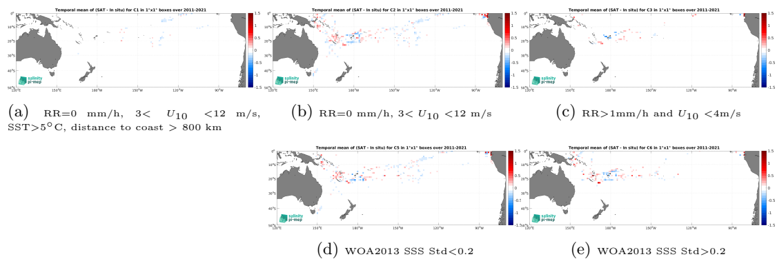
Figure 12: Temporal mean gridded over spatial boxes of size 1^\circ \times 1^\circ of \Delta SSS (SMAP SSS L4 OI v2 - Monthly (IPRC) - TSG (GOSUD-Research-vessel)) for 5 different subdatasets corresponding to:RR=0 mm/h, 3 < U_{10} < 12 m/s, SST >5^\circ\text{C} , distance to coast > 800 km (a), RR=0 mm/h, 3 < U_{10} < 12 m/s (b), RR >1 mm/h and U_{10} < 4 m/s (c), WOA2013 SSS Std <0.2 (d), WOA2013 SSS Std >0.2 (e).
