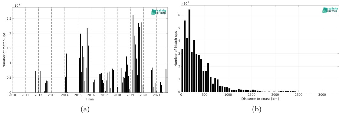
Figure 1: Number of match-ups between TSG (GOSUD-Research-vessel) and SMAP SSS L4 OI v2 - Monthly (IPRC) SSS as a function of time (a) and as function of the distance to coast (b) over the South Pacific Ocean Pi-MEP region and for the full satellite product period.
