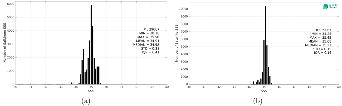
Figure 2: Histograms of SSS from Saildrone (a) and SMAP SSS L4 OI v2 - Monthly (IPRC) (b) considering all match-up pairs per bins of 0.1 over the South Pacific Ocean Pi-MEP region and for the full satellite product period.
