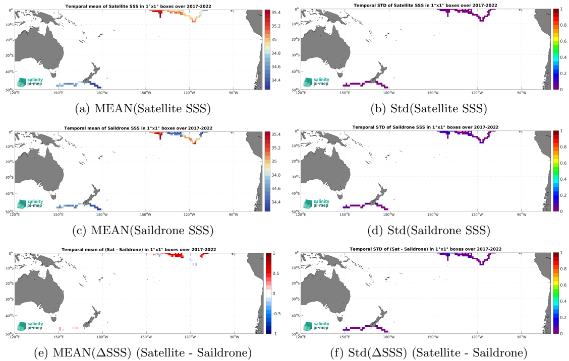
Figure 6: Temporal mean (left) and Std (right) of SSS from SMAP SSS L4 OI v2 - Monthly (IPRC) (top), Saildrone (middle), and of \Delta SSS (Satellite - Saildrone). Only match-up pairs are used to generate these maps.
