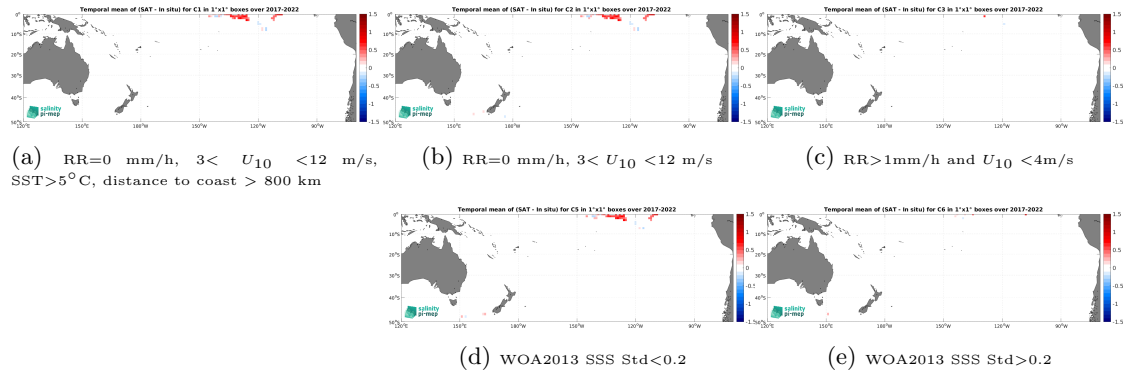
Figure 12: Temporal mean gridded over spatial boxes of size 1^\circ \times 1^\circ of \Delta SSS (SMAP SSS L4 OI v2 - Monthly (IPRC) - Saldrone) for 5 different subdatasets corresponding to:RR=0 mm/h, 3 < U_{10} < 12 m/s, SST >5^\circ C, distance to coast > 800 km (a), RR=0 mm/h, 3 < U_{10} < 12 m/s (b), RR >1 mm/h and U_{10} < 4 m/s (c), WOA2013 SSS Std <0.2 (d), WOA2013 SSS Std >0.2 (e).
