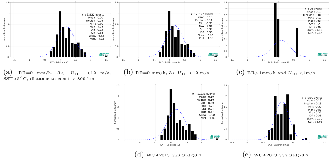
Figure 13: Normalized histogram of \Delta\text{SSS} (SMAP SSS L4 OI v2 - Monthly (IPRC) - Sairdron) for 5 different subdatasets corresponding to: RR=0 mm/h, 3 < U_{10} < 12 m/s, SST>5°C, distance to coast > 800 km (a), RR=0 mm/h, 3 < U_{10} < 12 m/s (b), RR>1mm/h and U_{10} < 4 m/s (c), WOA2013 SSS Std<0.2 (d), WOA2013 SSS Std>0.2 (e).
