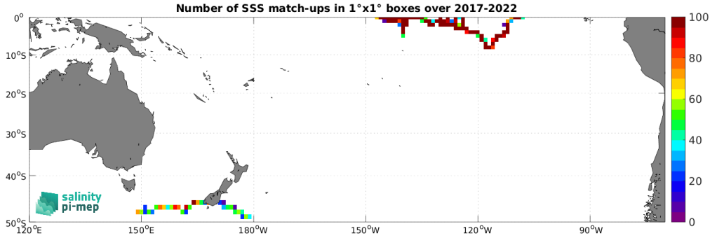
Figure 4: Number of SSS match-ups between Saildrone SSS and the SMAP SSS L4 OI v2 - Monthly (IPRC) SSS product for the South Pacific Ocean Pi-MEP region over 1^\circ \times 1^\circ boxes and for the full satellite product period.
