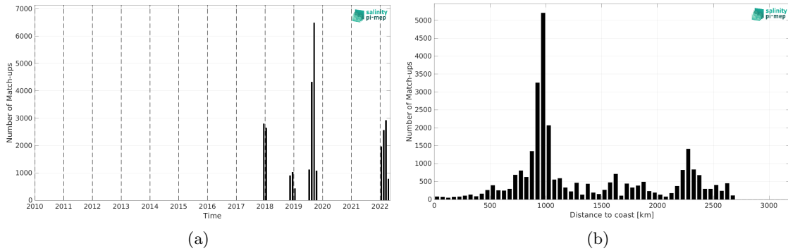
Figure 1: Number of match-ups between Saildrone and SMAP SSS L4 OI v2 - Monthly (IPRC) SSS as a function of time (a) and as function of the distance to coast (b) over the South Pacific Ocean Pi-MEP region and for the full satellite product period.
