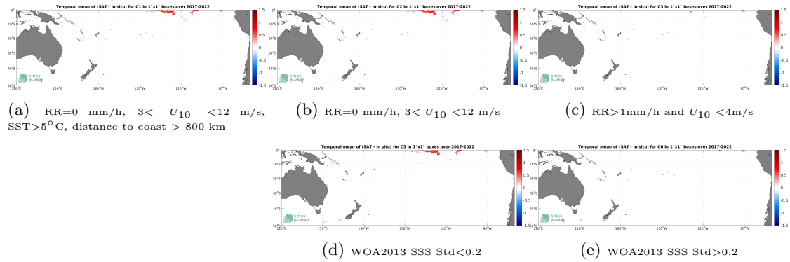
Figure 12: Temporal mean gridded over spatial boxes of size 1^\circ \times 1^\circ of \Delta SSS (SMAP SSS L4 OI v2 - Monthly (IPRC) - Saildrone) for 5 different subdatasets corresponding to:RR=0 mm/h, 3 < U_{10} < 12 m/s, SST >5^\circ C, distance to coast > 800 km (a), RR=0 mm/h, 3 < U_{10} < 12 m/s (b), RR >1 mm/h and U_{10} < 4 m/s (c), WOA2013 SSS Std <0.2 (d), WOA2013 SSS Std >0.2 (e).
