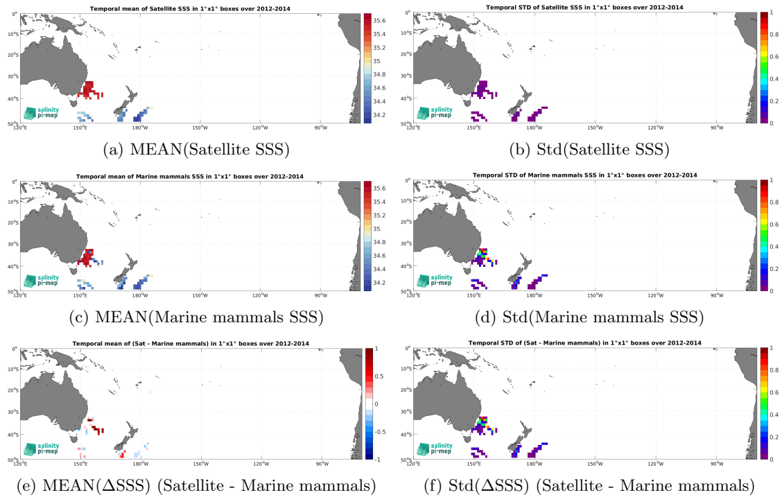
Figure 6: Temporal mean (left) and Std (right) of SSS from SMAP SSS L4 OI v2 - Monthly (IPRC) (top), Marine mammals (middle), and of \Delta SSS (Satellite - Marine mammals). Only match-up pairs are used to generate these maps.
