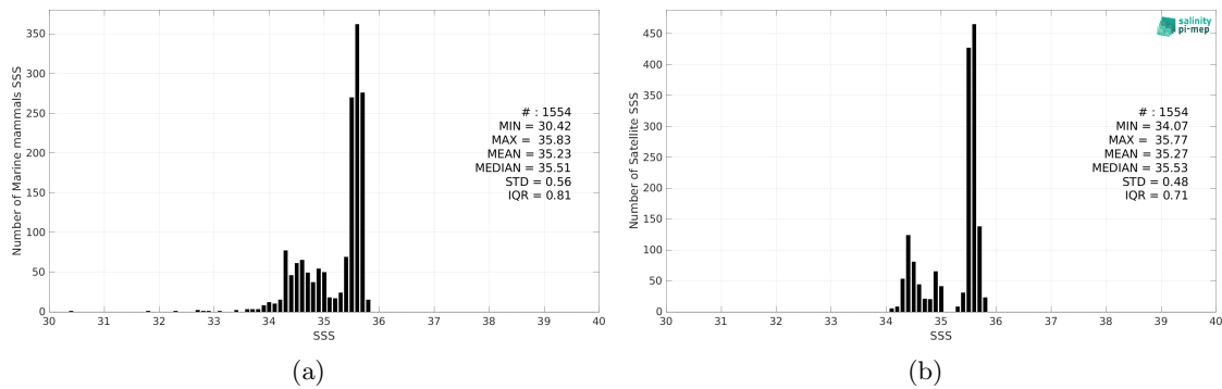
Figure 2: Histograms of SSS from Marine mammals (a) and SMAP SSS L4 OI v2 - Monthly (IPRC) (b) considering all match-up pairs per bins of 0.1 over the South Pacific Ocean Pi-MEP region and for the full satellite product period.
