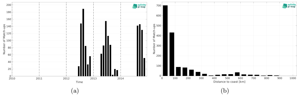
Figure 1: Number of match-ups between Marine mammals and SMAP SSS L4 OI v2 - Monthly (IPRC) SSS as a function of time (a) and as function of the distance to coast (b) over the South Pacific Ocean Pi-MEP region and for the full satellite product period.
