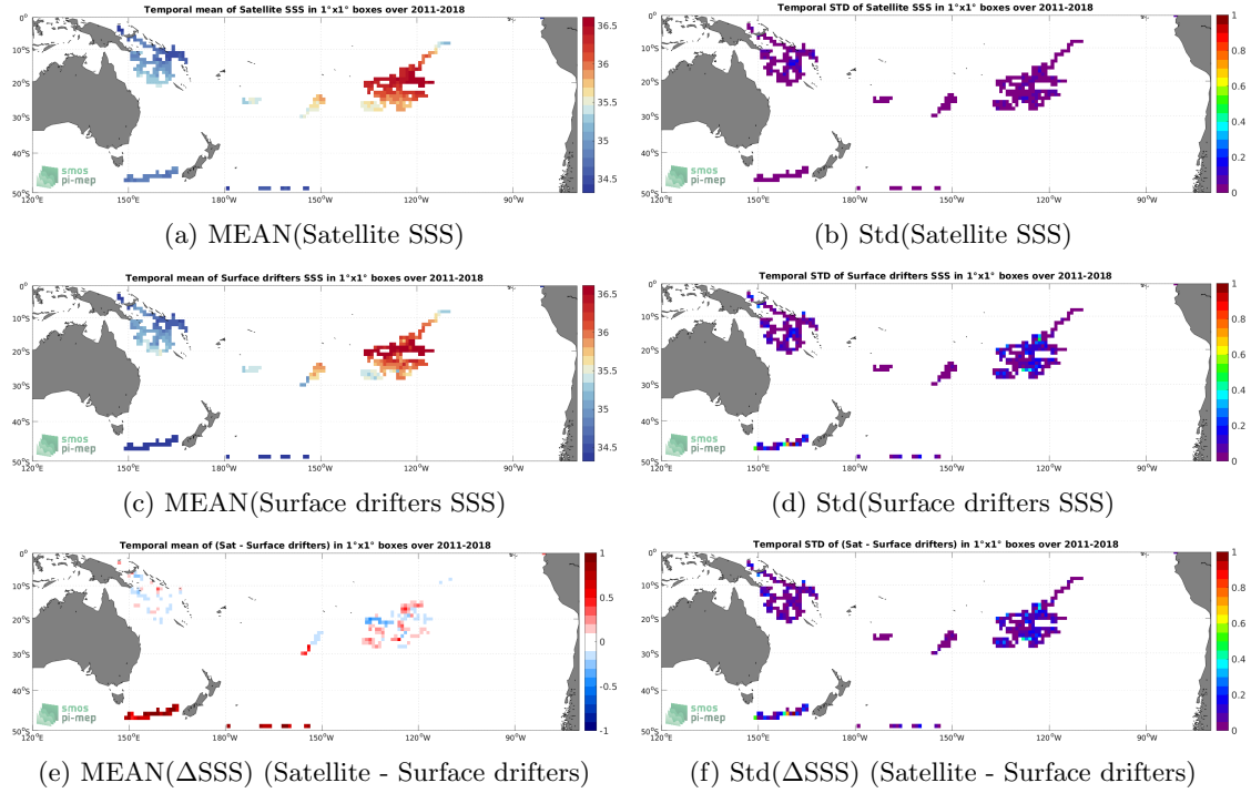
Figure 5: Temporal mean (left) and Std (right) of SSS from SMAP SSS L4 OI v2 - Monthly (IPRC) (top), Surface drifters (middle), and of \Delta SSS (Satellite - Surface drifters). Only match-up pairs are used to generate these maps.
