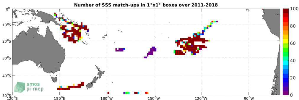
Figure 3: Number of SSS match-ups between Surface drifters SSS and the SMAP SSS L4 OI v2 - Monthly (IPRC) SSS product for the South Pacific Ocean Pi-MEP region over 1^\circ \times 1^\circ boxes and for the full satellite product period.
