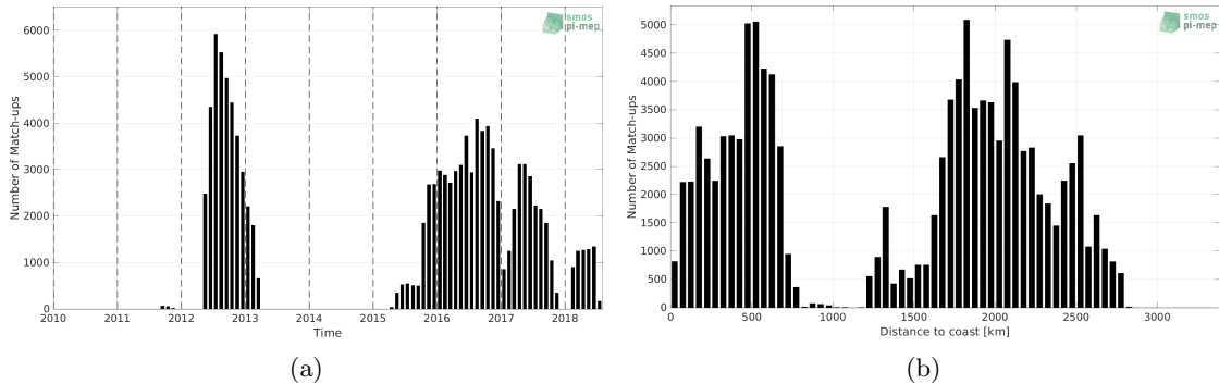
Figure 1: Number of match-ups between Surface drifters and SMAP SSS L4 OI v2 - Monthly (IPRC) SSS as a function of time (a) and as function of the distance to coast (b) over the South Pacific Ocean Pi-MEP region and for the full satellite product period.
