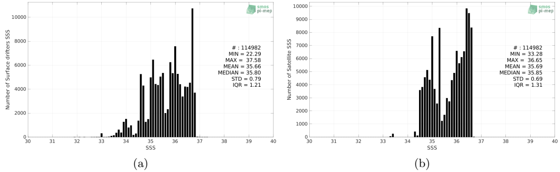
Figure 2: Histograms of SSS from Surface drifters (a) and SMAP SSS L4 OI v2 - Monthly (IPRC) (b) considering all match-up pairs per bins of 0.1 over the South Pacific Ocean Pi-MEP region and for the full satellite product period.
