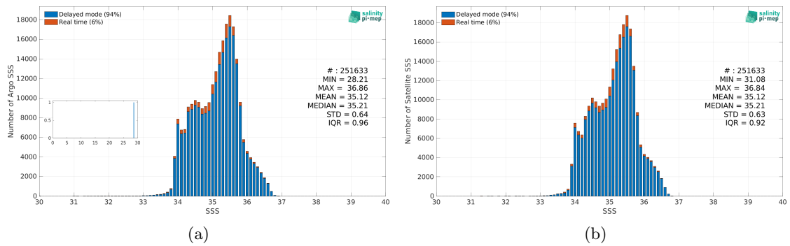
Figure 2: Histograms of SSS from Argo (a) and SMAP SSS L4 OI v2 - Monthly (IPRC) (b) considering all match-up pairs per bins of 0.1 over the South Pacific Ocean Pi-MEP region and for the full satellite product period.
