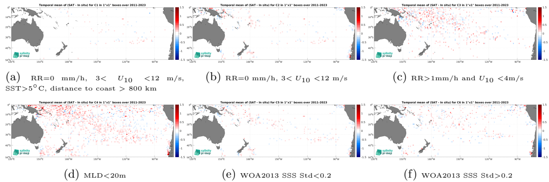
Figure 12: Temporal mean gridded over spatial boxes of size 1^\circ \times 1^\circ of \Delta SSS (SMAP SSS L4 OI v2 - Monthly (IPRC) - Argo) for 6 different subdatasets corresponding to:RR=0 mm/h, 3 < U_{10} < 12 m/s, SST >5^\circ\text{C} , distance to coast > 800 km (a), RR=0 mm/h, 3 < U_{10} < 12 m/s (b), RR >1 mm/h and U_{10} < 4 m/s (c),MLD <20 m (d),WOA2013 SSS Std <0.2 (e),WOA2013 SSS Std >0.2 (f).
