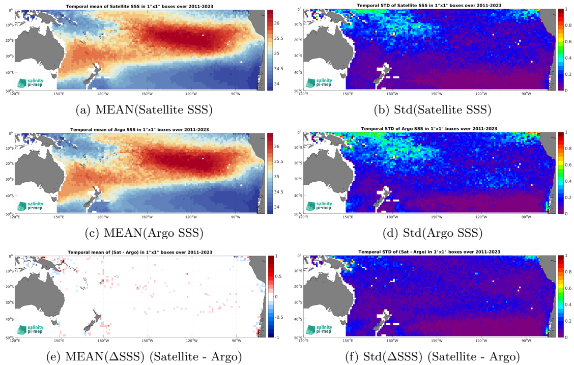
Figure 6: Temporal mean (left) and Std (right) of SSS from SMAP SSS L4 OI v2 - Monthly (IPRC) (top), Argo (middle), and of \Delta SSS (Satellite - Argo). Only match-up pairs are used to generate these maps.
