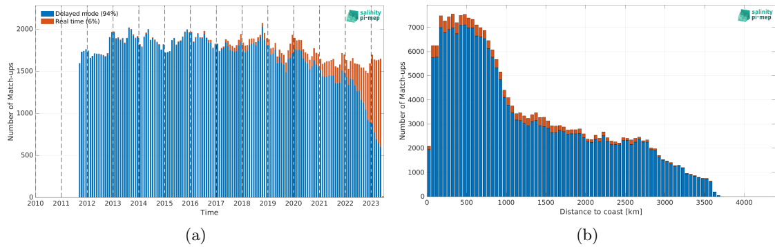
Figure 1: Number of match-ups between Argo and SMAP SSS L4 OI v2 - Monthly (IPRC) SSS as a function of time (a) and as function of the distance to coast (b) over the South Pacific Ocean Pi-MEP region and for the full satellite product period.
