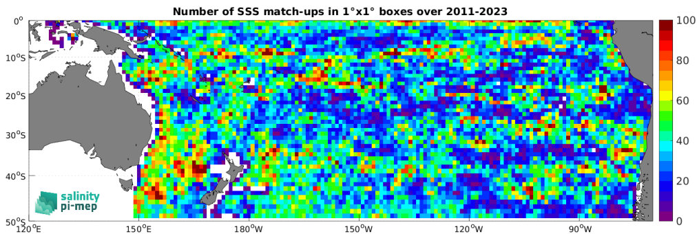
Figure 4: Number of SSS match-ups between Argo SSS and the SMAP SSS L4 OI v2 - Monthly (IPRC) SSS product for the South Pacific Ocean Pi-MEP region over 1^\circ \times 1^\circ boxes and for the full satellite product period.
