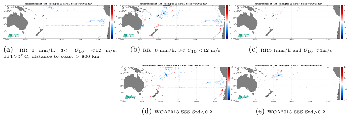
Figure 14: Temporal mean gridded over spatial boxes of size 1^\circ \times 1^\circ of \Delta SSS (SMAP SSS L3 v6 - 8-Day running (RSS) - TSG (SAMOS)) for 5 different subdatasets corresponding to: RR=0 mm/h, 3 < U_{10} < 12 m/s, SST > 5^\circ\text{C} , distance to coast > 800 km (a), RR=0 mm/h, 3 < U_{10} < 12 m/s (b), RR > 1 mm/h and U_{10} < 4 m/s (c), WOA2013 SSS Std < 0.2 (d), WOA2013 SSS Std > 0.2 (e).
