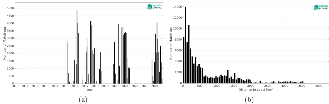
Figure 2: Number of match-ups between TSG (SAMOS) and SMAP SSS L3 v6 - 8-Day running (RSS) SSS as a function of time (a) and as function of the distance to coast (b) over the South Pacific Ocean Pi-MEP region and for the full satellite product period.
