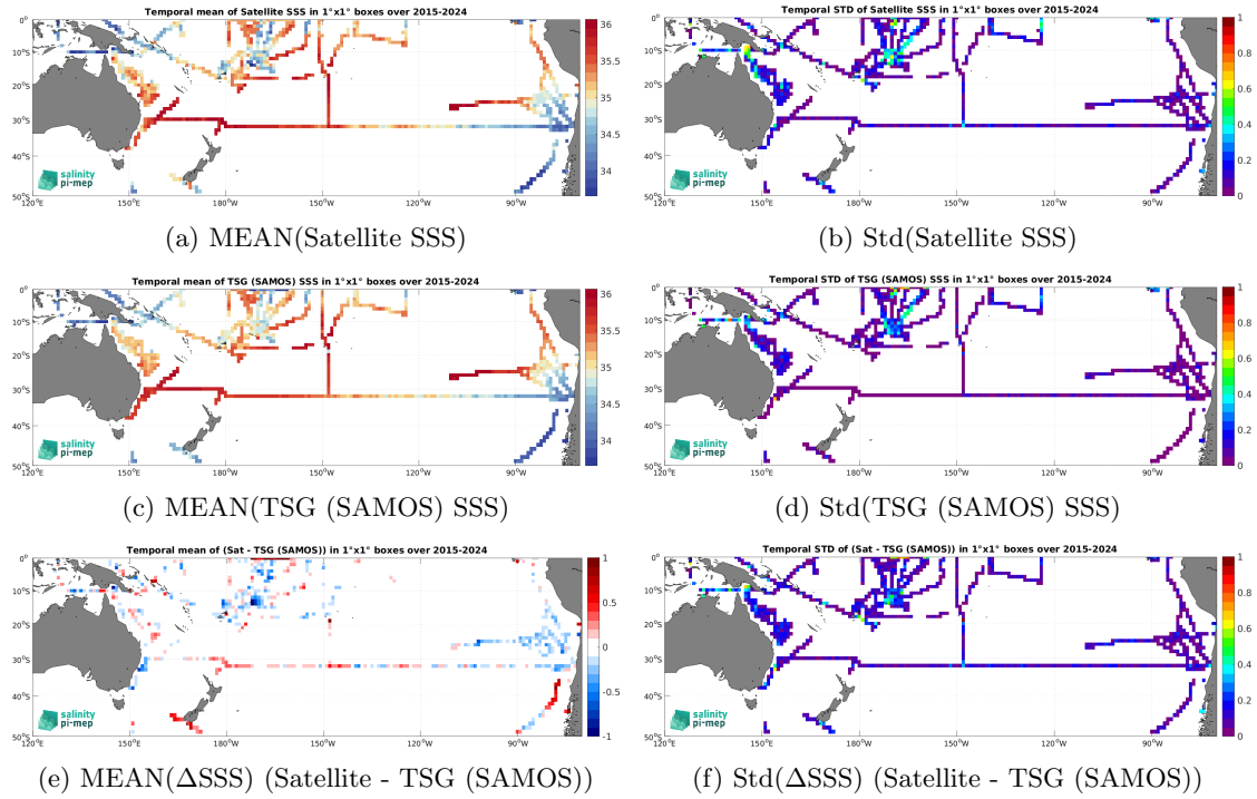
Figure 7: Temporal mean (left) and Std (right) of SSS from SMAP SSS L3 v6 - 8-Day running (RSS) (top), TSG (SAMOS) (middle), and of \Delta SSS (Satellite - TSG (SAMOS)). Only match-up pairs are used to generate these maps.
