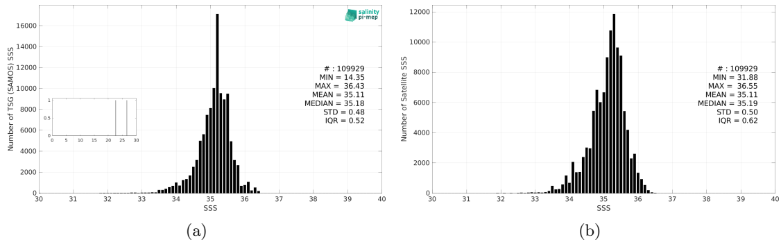
Figure 3: Histograms of SSS from TSG (SAMOS) (a) and SMAP SSS L3 v6 - 8-Day running (RSS) (b) considering all match-up pairs per bins of 0.1 over the South Pacific Ocean Pi-MEP region and for the full satellite product period.
