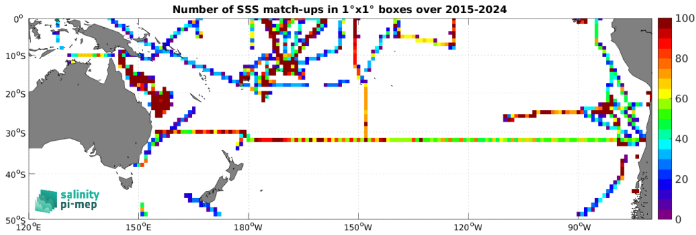
Figure 5: Number of SSS match-ups between TSG (SAMOS) SSS and the SMAP SSS L3 v6 - 8-Day running (RSS) SSS product for the South Pacific Ocean Pi-MEP region over 1^\circ \times 1^\circ boxes and for the full satellite product period.
