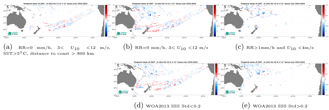
Figure 14: Temporal mean gridded over spatial boxes of size 1^\circ \times 1^\circ of \Delta SSS (SMAP SSS L3 v6 - 8-Day running (RSS) - TSG (LEGOS-DM)) for 5 different subdatasets corresponding to:RR=0 mm/h, 3 < U_{10} < 12 m/s, SST >5^\circ\text{C} , distance to coast > 800 km (a), RR=0 mm/h, 3 < U_{10} < 12 m/s (b), RR >1 mm/h and U_{10} < 4 m/s (c), WOA2013 SSS Std <0.2 (d), WOA2013 SSS Std >0.2 (e).
