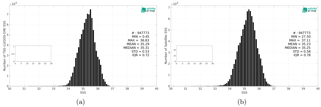
Figure 3: Histograms of SSS from TSG (LEGOS-DM) (a) and SMAP SSS L3 v6 - 8-Day running (RSS) (b) considering all match-up pairs per bins of 0.1 over the South Pacific Ocean Pi-MEP region and for the full satellite product period.
