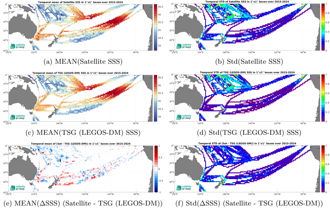
Figure 7: Temporal mean (left) and Std (right) of SSS from SMAP SSS L3 v6 - 8-Day running (RSS) (top), TSG (LEGOS-DM) (middle), and of \Delta SSS (Satellite - TSG (LEGOS-DM)). Only match-up pairs are used to generate these maps.
