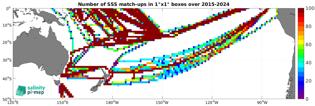
Figure 5: Number of SSS match-ups between TSG (LEGOS-DM) SSS and the SMAP SSS L3 v6 - 8-Day running (RSS) SSS product for the South Pacific Ocean Pi-MEP region over 1^\circ \times 1^\circ boxes and for the full satellite product period.
