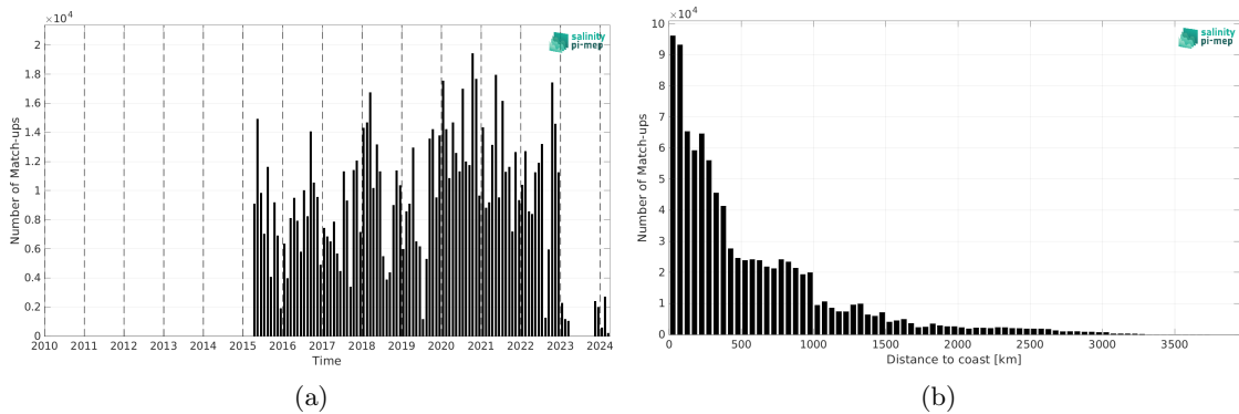
Figure 2: Number of match-ups between TSG (LEGOS-DM) and SMAP SSS L3 v6 - 8-Day running (RSS) SSS as a function of time (a) and as function of the distance to coast (b) over the South Pacific Ocean Pi-MEP region and for the full satellite product period.
