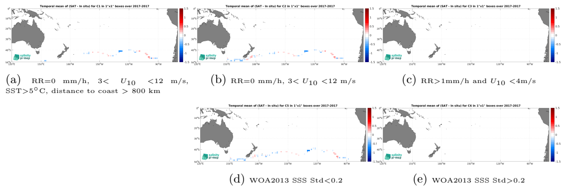
Figure 14: Temporal mean gridded over spatial boxes of size 1^\circ \times 1^\circ of \Delta SSS (SMAP SSS L3 v6 - 8-Day running (RSS) - TSG (GOSUD-Sailing-ship)) for 5 different subdatasets corresponding to:RR=0 mm/h, 3 < U_{10} < 12 m/s, SST>5°C, distance to coast > 800 km (a), RR=0 mm/h, 3 < U_{10} < 12 m/s (b), RR>1mm/h and U_{10} < 4 m/s (c), WOA2013 SSS Std<0.2 (d), WOA2013 SSS Std>0.2 (e).
