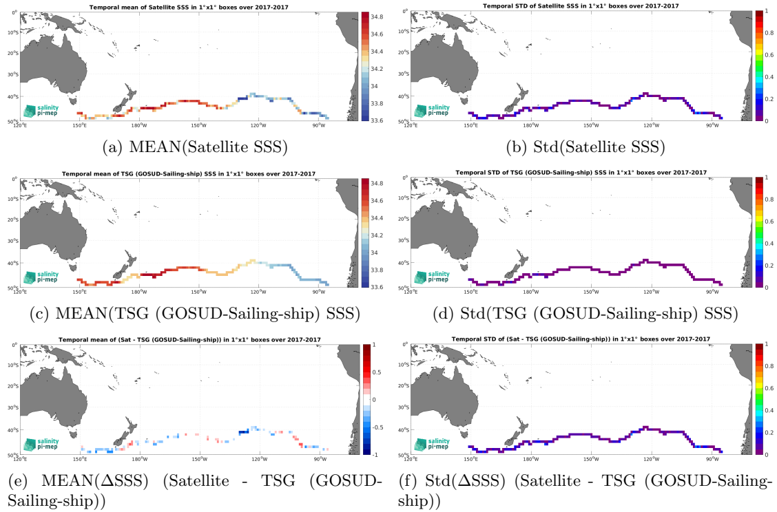
Figure 7: Temporal mean (left) and Std (right) of SSS from SMAP SSS L3 v6 - 8-Day running (RSS) (top), TSG (GOSUD-Sailing-ship) (middle), and of \Delta SSS (Satellite - TSG (GOSUD-Sailing-ship)). Only match-up pairs are used to generate these maps.
