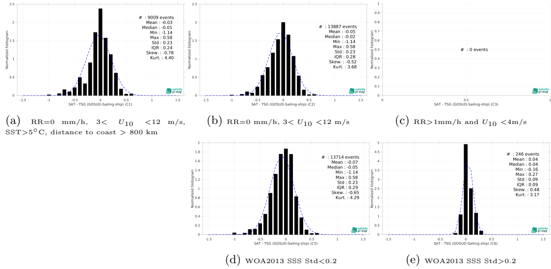
Figure 15: Normalized histogram of \Delta\text{SSS} (SMAP SSS L3 v6 - 8-Day running (RSS) - TSG (GOSUD-Sailing-ship)) for 5 different subdatasets corresponding to: RR=0 mm/h, 3 < U_{10} < 12 m/s, SST >5^{\circ}\text{C} , distance to coast > 800 km (a), RR=0 mm/h, 3 < U_{10} < 12 m/s (b), RR >1 mm/h and U_{10} < 4 m/s (c), WOA2013 SSS Std <0.2 (d), WOA2013 SSS Std >0.2 (e).
