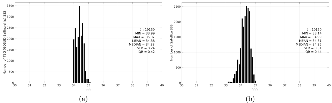
Figure 3: Histograms of SSS from TSG (GOSUD-Sailing-ship) (a) and SMAP SSS L3 v6 - 8-Day running (RSS) (b) considering all match-up pairs per bins of 0.1 over the South Pacific Ocean Pi-MEP region and for the full satellite product period.
