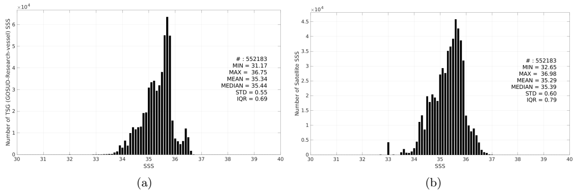
Figure 3: Histograms of SSS from TSG (GOSUD-Research-vessel) (a) and SMAP SSS L3 v6 - 8-Day running (RSS) (b) considering all match-up pairs per bins of 0.1 over the South Pacific Ocean Pi-MEP region and for the full satellite product period.
