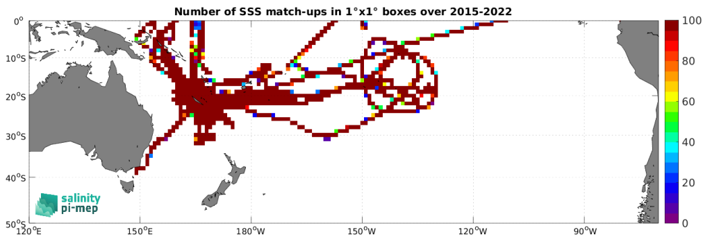
Figure 5: Number of SSS match-ups between TSG (GOSUD-Research-vessel) SSS and the SMAP SSS L3 v6 - 8-Day running (RSS) SSS product for the South Pacific Ocean Pi-MEP region over 1^\circ \times 1^\circ boxes and for the full satellite product period.
