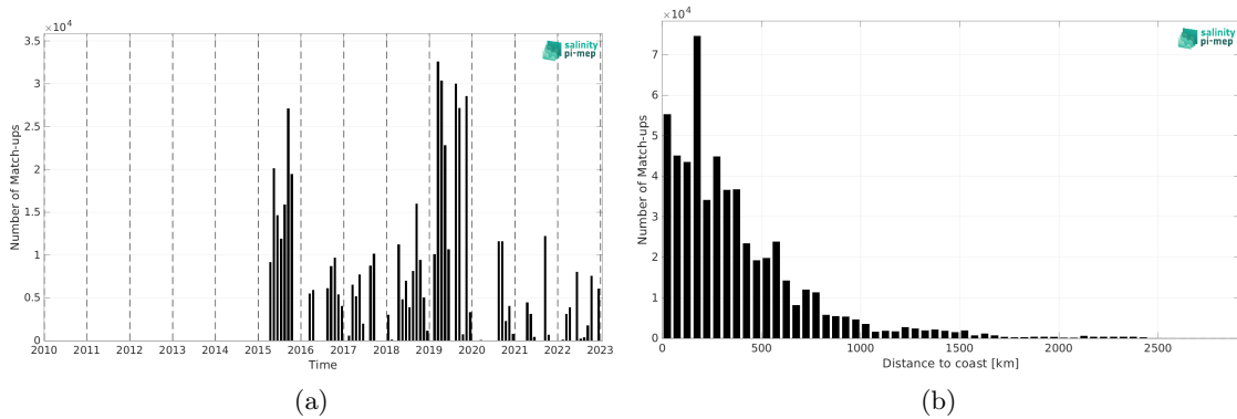
Figure 2: Number of match-ups between TSG (GOSUD-Research-vessel) and SMAP SSS L3 v6 - 8-Day running (RSS) SSS as a function of time (a) and as function of the distance to coast (b) over the South Pacific Ocean Pi-MEP region and for the full satellite product period.
