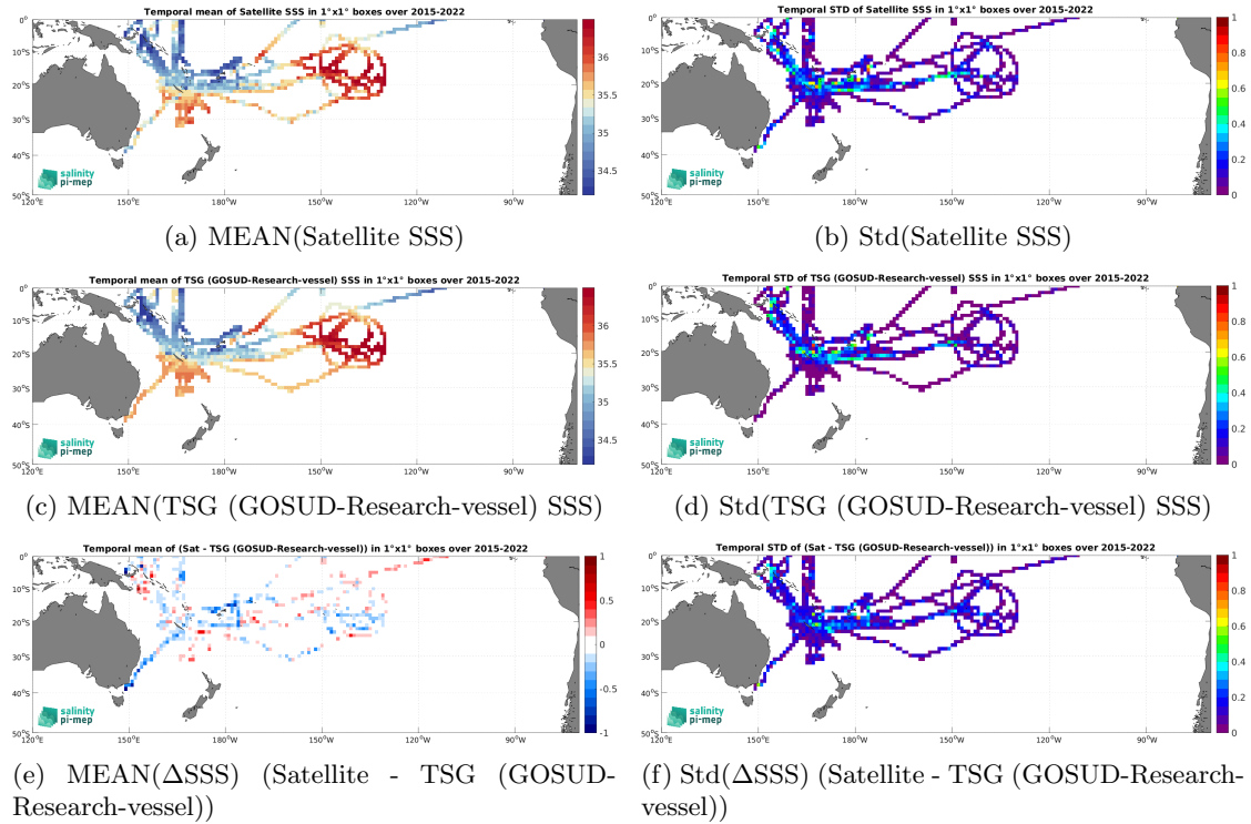
Figure 7: Temporal mean (left) and Std (right) of SSS from SMAP SSS L3 v6 - 8-Day running (RSS) (top), TSG (GOSUD-Research-vessel) (middle), and of \Delta SSS (Satellite - TSG (GOSUD-Research-vessel)). Only match-up pairs are used to generate these maps.
