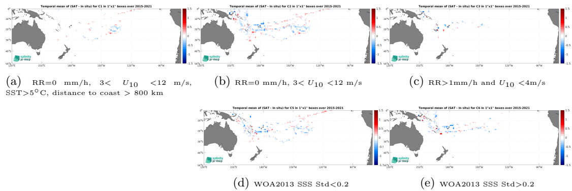
Figure 14: Temporal mean gridded over spatial boxes of size 1^\circ \times 1^\circ of \Delta\text{SSS} (SMAP SSS L3 v6 - 8-Day running (RSS) - TSG (GOSUD-Research-vessel)) for 5 different subdatasets corresponding to:RR=0 mm/h, 3 < U_{10} < 12 m/s, SST>5°C, distance to coast > 800 km (a), RR=0 mm/h, 3 < U_{10} < 12 m/s (b), RR>1mm/h and U_{10} < 4 m/s (c), WOA2013 SSS Std<0.2 (d), WOA2013 SSS Std>0.2 (e).
