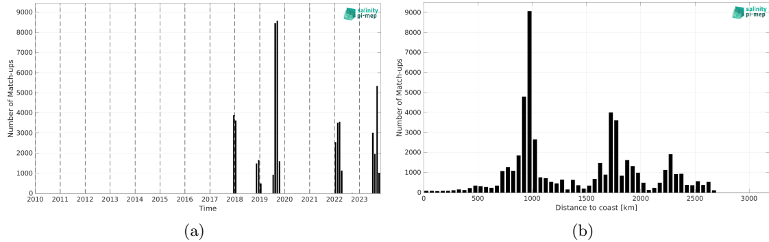
Figure 2: Number of match-ups between Saildrone and SMAP SSS L3 v6 - 8-Day running (RSS) SSS as a function of time (a) and as function of the distance to coast (b) over the South Pacific Ocean Pi-MEP region and for the full satellite product period.
