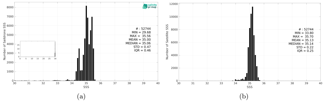
Figure 3: Histograms of SSS from Saildrone (a) and SMAP SSS L3 v6 - 8-Day running (RSS) (b) considering all match-up pairs per bins of 0.1 over the South Pacific Ocean Pi-MEP region and for the full satellite product period.
