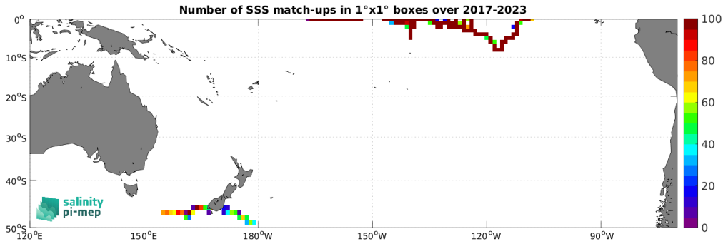
Figure 5: Number of SSS match-ups between Saildrone SSS and the SMAP SSS L3 v6 - 8-Day running (RSS) SSS product for the South Pacific Ocean Pi-MEP region over 1^\circ \times 1^\circ boxes and for the full satellite product period.
