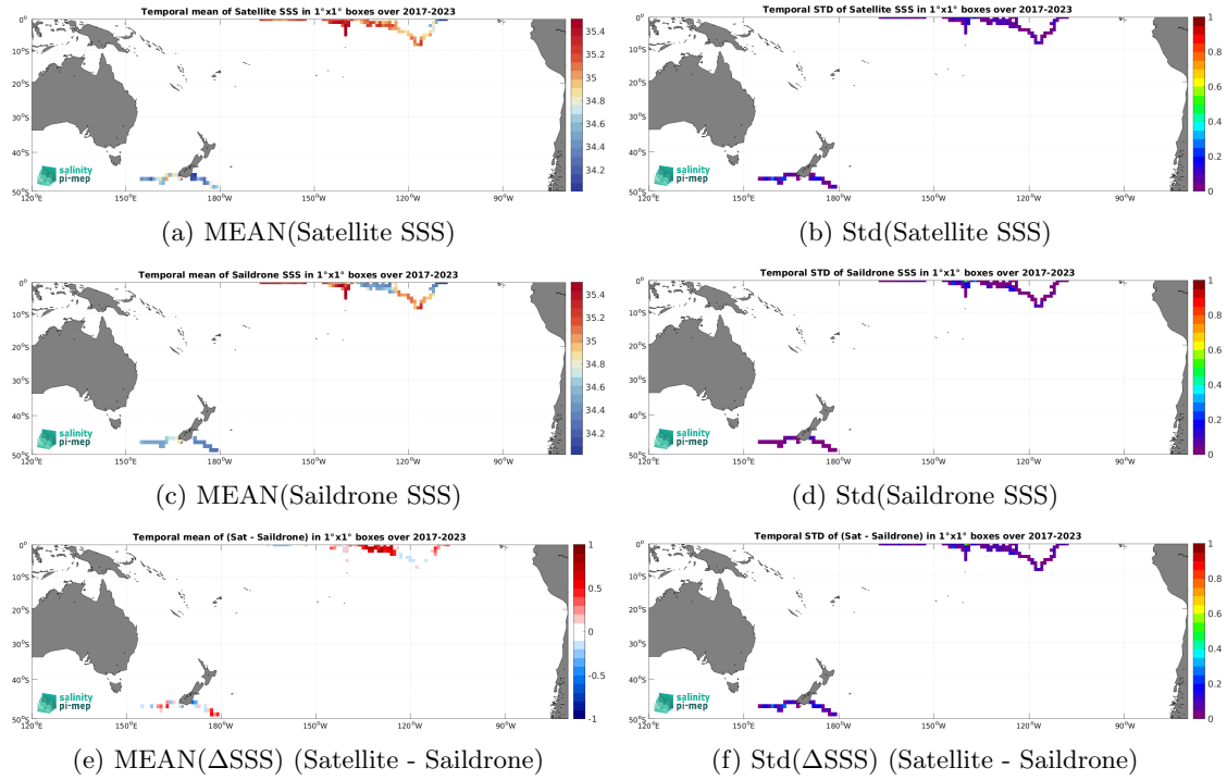
Figure 7: Temporal mean (left) and Std (right) of SSS from SMAP SSS L3 v6 - 8-Day running (RSS) (top), Saildrone (middle), and of \Delta SSS (Satellite - Saildrone). Only match-up pairs are used to generate these maps.
