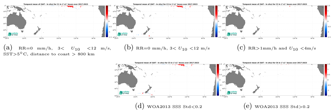
Figure 14: Temporal mean gridded over spatial boxes of size 1^\circ \times 1^\circ of \Delta\text{SSS} (SMAP SSS L3 v6 - 8-Day running (RSS) - Saifdrone) for 5 different subdatasets corresponding to:RR=0 mm/h, 3 < U_{10} < 12 m/s, SST>5°C, distance to coast > 800 km (a), RR=0 mm/h, 3 < U_{10} < 12 m/s (b), RR>1mm/h and U_{10} < 4 m/s (c), WOA2013 SSS Std<0.2 (d), WOA2013 SSS Std>0.2 (e).
