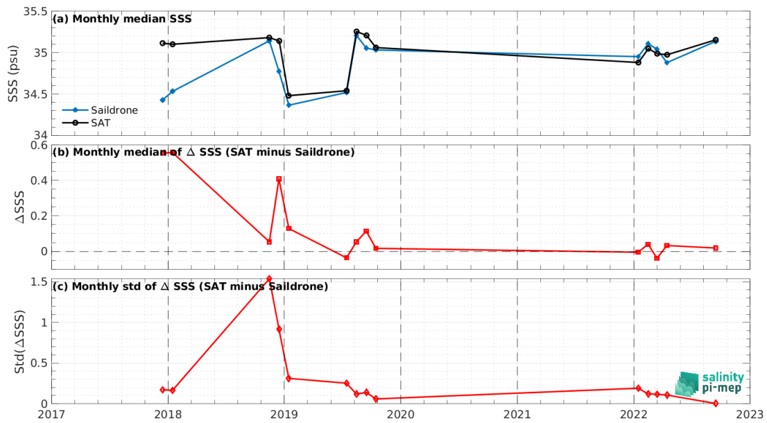
Figure 8: Time series of the monthly median SSS (top), median of \Delta SSS (Satellite - Sairdrone) and Std(\Delta SSS) (Satellite - Sairdrone) over the South Pacific Ocean Pi-MEP region considering all match-ups collected by the Pi-MEP.
