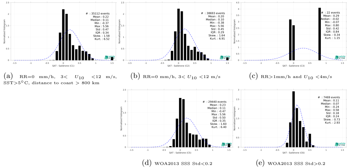
Figure 15: Normalized histogram of \Delta SSS (SMAP SSS L3 v6 - 8-Day running (RSS) - Sairdrome) for 5 different subdatasets corresponding to: RR=0 mm/h, 3 < U_{10} < 12 m/s, SST>5°C, distance to coast > 800 km (a), RR=0 mm/h, 3 < U_{10} < 12 m/s (b), RR>1mm/h and U_{10} < 4 m/s (c), WOA2013 SSS Std<0.2 (d), WOA2013 SSS Std>0.2 (e).
