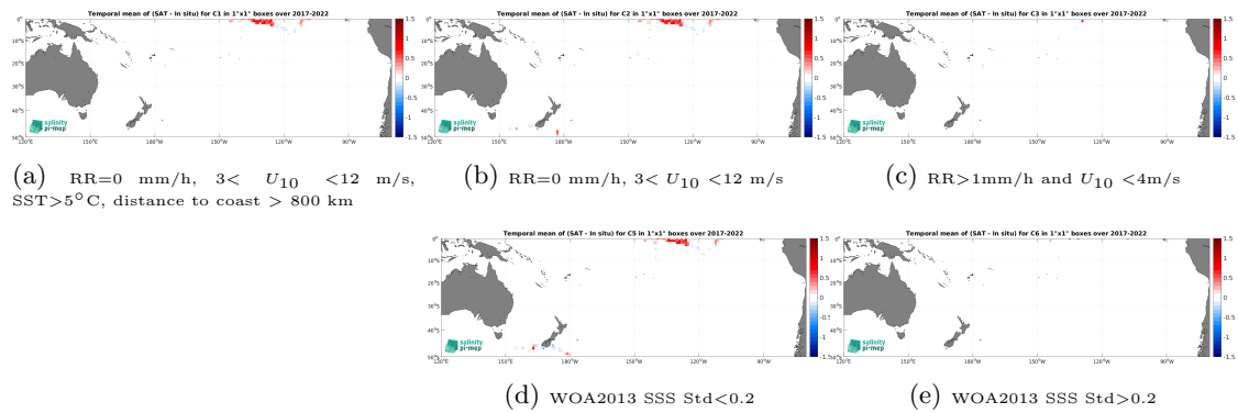
Figure 14: Temporal mean gridded over spatial boxes of size 1^\circ \times 1^\circ of \Delta\text{SSS} (SMAP SSS L3 v6 - 8-Day running (RSS) - Saildrone) for 5 different subdatasets corresponding to:RR=0 mm/h, 3 < U_{10} < 12 m/s, SST >5^\circ\text{C} , distance to coast > 800 km (a), RR=0 mm/h, 3 < U_{10} < 12 m/s (b), RR >1 mm/h and U_{10} < 4 m/s (c), WOA2013 SSS Std <0.2 (d), WOA2013 SSS Std >0.2 (e).
