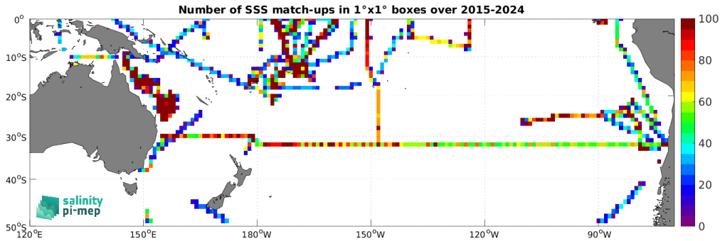
Figure 5: Number of SSS match-ups between TSG (SAMOS) SSS and the SMAP SSS L3 v6 - Monthly (RSS) SSS product for the South Pacific Ocean Pi-MEP region over 1^\circ \times 1^\circ boxes and for the full satellite product period.
