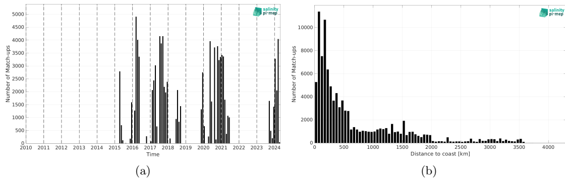
Figure 2: Number of match-ups between TSG (SAMOS) and SMAP SSS L3 v6 - Monthly (RSS) SSS as a function of time (a) and as function of the distance to coast (b) over the South Pacific Ocean Pi-MEP region and for the full satellite product period.
