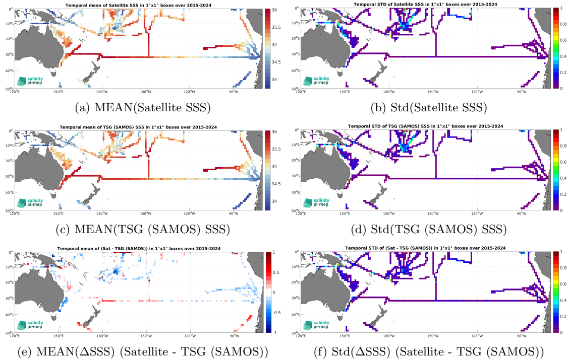
Figure 7: Temporal mean (left) and Std (right) of SSS from SMAP SSS L3 v6 - Monthly (RSS) (top), TSG (SAMOS) (middle), and of \Delta SSS (Satellite - TSG (SAMOS)). Only match-up pairs are used to generate these maps.
