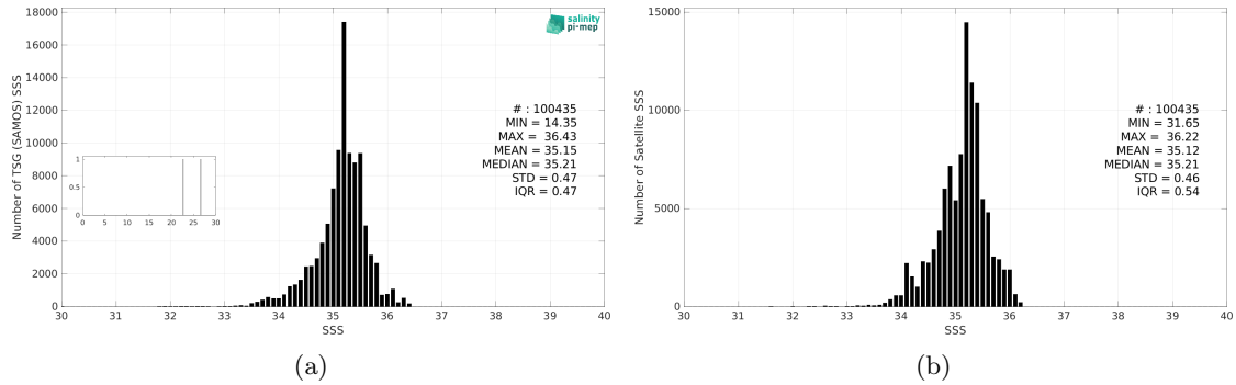
Figure 3: Histograms of SSS from TSG (SAMOS) (a) and SMAP SSS L3 v6 - Monthly (RSS) (b) considering all match-up pairs per bins of 0.1 over the South Pacific Ocean Pi-MEP region and for the full satellite product period.
