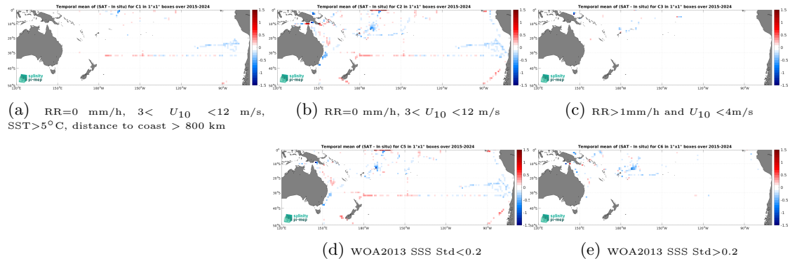
Figure 14: Temporal mean gridded over spatial boxes of size 1^\circ \times 1^\circ of \Delta\text{SSS} (SMAP SSS L3 v6 - Monthly (RSS) - TSG (SAMOS)) for 5 different subdatasets corresponding to:RR=0 mm/h, 3 < U_{10} < 12 m/s, SST >5^\circ\text{C} , distance to coast > 800 km (a), RR=0 mm/h, 3 < U_{10} < 12 m/s (b), RR >1 mm/h and U_{10} < 4 m/s (c), WOA2013 SSS Std <0.2 (d), WOA2013 SSS Std >0.2 (e).
