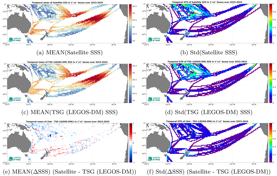
Figure 7: Temporal mean (left) and Std (right) of SSS from SMAP SSS L3 v6 - Monthly (RSS) (top), TSG (LEGOS-DM) (middle), and of \Delta SSS (Satellite - TSG (LEGOS-DM)). Only match-up pairs are used to generate these maps.
