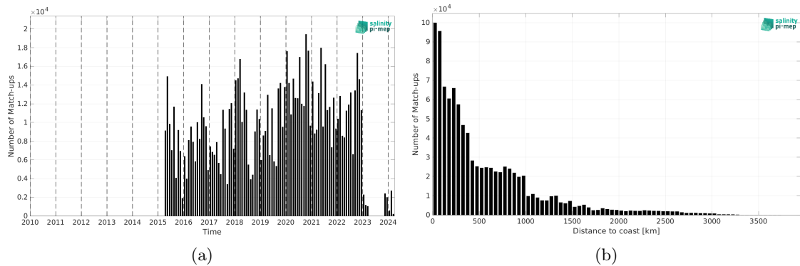
Figure 2: Number of match-ups between TSG (LEGOS-DM) and SMAP SSS L3 v6 - Monthly (RSS) SSS as a function of time (a) and as function of the distance to coast (b) over the South Pacific Ocean Pi-MEP region and for the full satellite product period.
