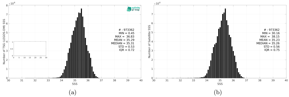
Figure 3: Histograms of SSS from TSG (LEGOS-DM) (a) and SMAP SSS L3 v6 - Monthly (RSS) (b) considering all match-up pairs per bins of 0.1 over the South Pacific Ocean Pi-MEP region and for the full satellite product period.
