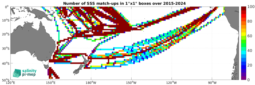
Figure 5: Number of SSS match-ups between TSG (LEGOS-DM) SSS and the SMAP SSS L3 v6 - Monthly (RSS) SSS product for the South Pacific Ocean Pi-MEP region over 1^\circ \times 1^\circ boxes and for the full satellite product period.
