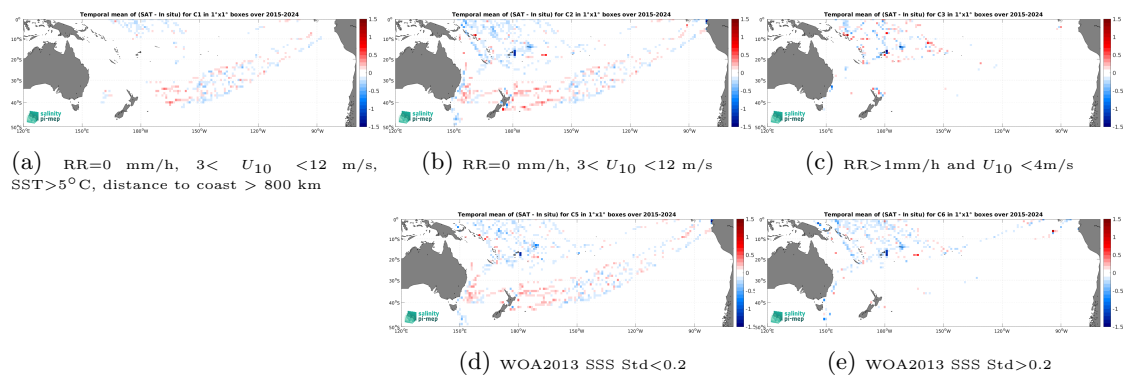
Figure 14: Temporal mean gridded over spatial boxes of size 1^\circ \times 1^\circ of \Delta\text{SSS} (SMAP SSS L3 v6 - Monthly (RSS) - TSG (LEGOS-DM)) for 5 different subdatasets corresponding to:RR=0 mm/h, 3 < U_{10} < 12 m/s, SST >5^\circ\text{C} , distance to coast > 800 km (a), RR=0 mm/h, 3 < U_{10} < 12 m/s (b), RR >1 mm/h and U_{10} < 4 m/s (c), WOA2013 SSS Std <0.2 (d), WOA2013 SSS Std >0.2 (e).
