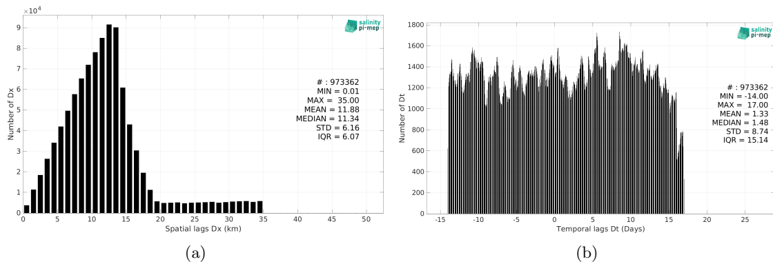
Figure 6: Histograms of the spatial (a) and temporal (b) lags between the location/time of the TSG (LEGOS-DM) measurement and the date of the corresponding SMAP SSS L3 v6 - Monthly (RSS) SSS pixel.
