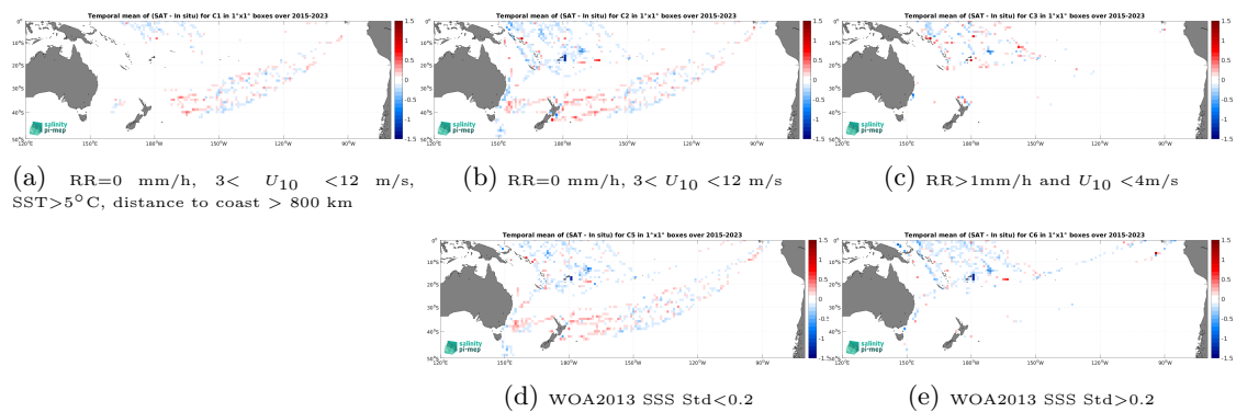
Figure 14: Temporal mean gridded over spatial boxes of size 1^\circ \times 1^\circ of \Delta SSS (SMAP SSS L3 v6 - Monthly (RSS) - TSG (LEGOS-DM)) for 5 different subdatasets corresponding to:RR=0 mm/h, 3 < U_{10} < 12 m/s, SST >5^\circ\text{C} , distance to coast > 800 km (a), RR=0 mm/h, 3 < U_{10} < 12 m/s (b), RR >1 mm/h and U_{10} < 4 m/s (c), WOA2013 SSS Std <0.2 (d), WOA2013 SSS Std >0.2 (e).
