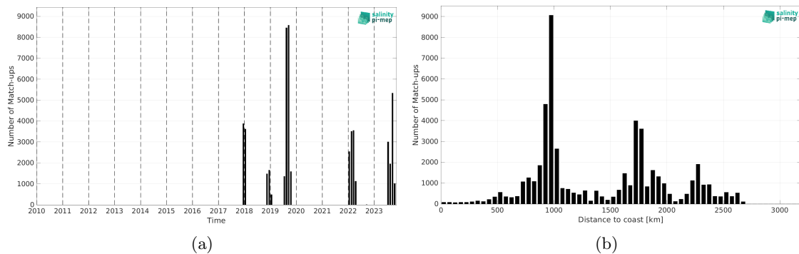
Figure 2: Number of match-ups between Sairdrone and SMAP SSS L3 v6 - Monthly (RSS) SSS as a function of time (a) and as function of the distance to coast (b) over the South Pacific Ocean Pi-MEP region and for the full satellite product period.
