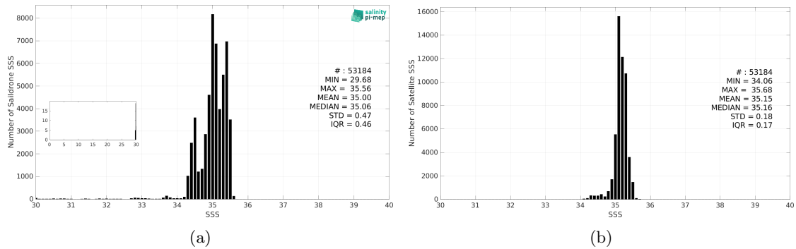
Figure 3: Histograms of SSS from Saildrone (a) and SMAP SSS L3 v6 - Monthly (RSS) (b) considering all match-up pairs per bins of 0.1 over the South Pacific Ocean Pi-MEP region and for the full satellite product period.
