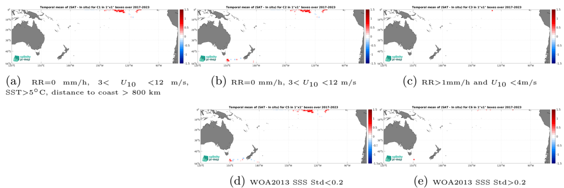
Figure 14: Temporal mean gridded over spatial boxes of size 1^\circ \times 1^\circ of \Delta\text{SSS} (SMAP SSS L3 v6 - Monthly (RSS) - Saildrone) for 5 different subdatasets corresponding to:RR=0 mm/h, 3 < U_{10} < 12 m/s, SST >5^\circ\text{C} , distance to coast > 800 km (a), RR=0 mm/h, 3 < U_{10} < 12 m/s (b), RR >1 mm/h and U_{10} < 4 m/s (c), WOA2013 SSS Std <0.2 (d), WOA2013 SSS Std >0.2 (e).
