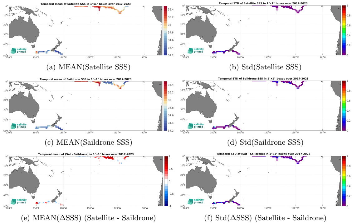
Figure 7: Temporal mean (left) and Std (right) of SSS from SMAP SSS L3 v6 - Monthly (RSS) (top), Saildrone (middle), and of \Delta SSS (Satellite - Saildrone). Only match-up pairs are used to generate these maps.
