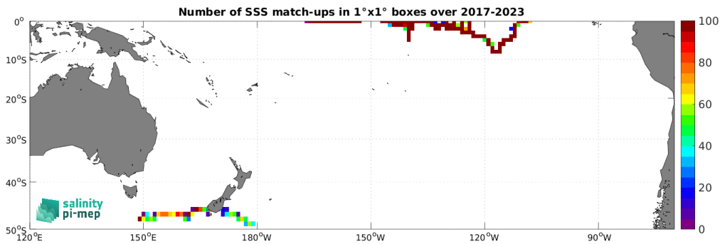
Figure 5: Number of SSS match-ups between Saildrone SSS and the SMAP SSS L3 v6 - Monthly (RSS) SSS product for the South Pacific Ocean Pi-MEP region over 1^\circ \times 1^\circ boxes and for the full satellite product period.
