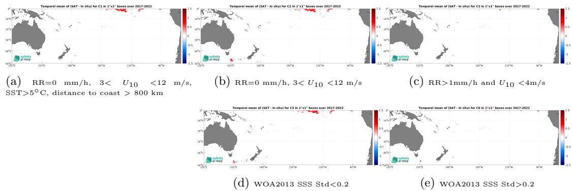
Figure 14: Temporal mean gridded over spatial boxes of size 1^\circ \times 1^\circ of \Delta SSS (SMAP SSS L3 v6 - Monthly (RSS) - Saildrone) for 5 different subdatasets corresponding to:RR=0 mm/h, 3 < U_{10} < 12 m/s, SST > 5^\circ C , distance to coast > 800 km (a), RR=0 mm/h, 3 < U_{10} < 12 m/s (b), RR >1 mm/h and U_{10} < 4 m/s (c), WOA2013 SSS Std <0.2 (d), WOA2013 SSS Std >0.2 (e).
