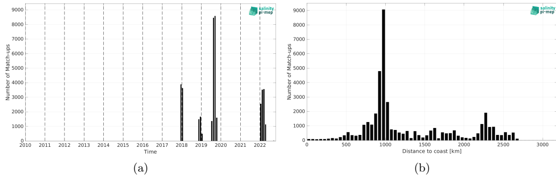
Figure 2: Number of match-ups between Saildrone and SMAP SSS L3 v6 - Monthly (RSS) SSS as a function of time (a) and as function of the distance to coast (b) over the South Pacific Ocean Pi-MEP region and for the full satellite product period.
