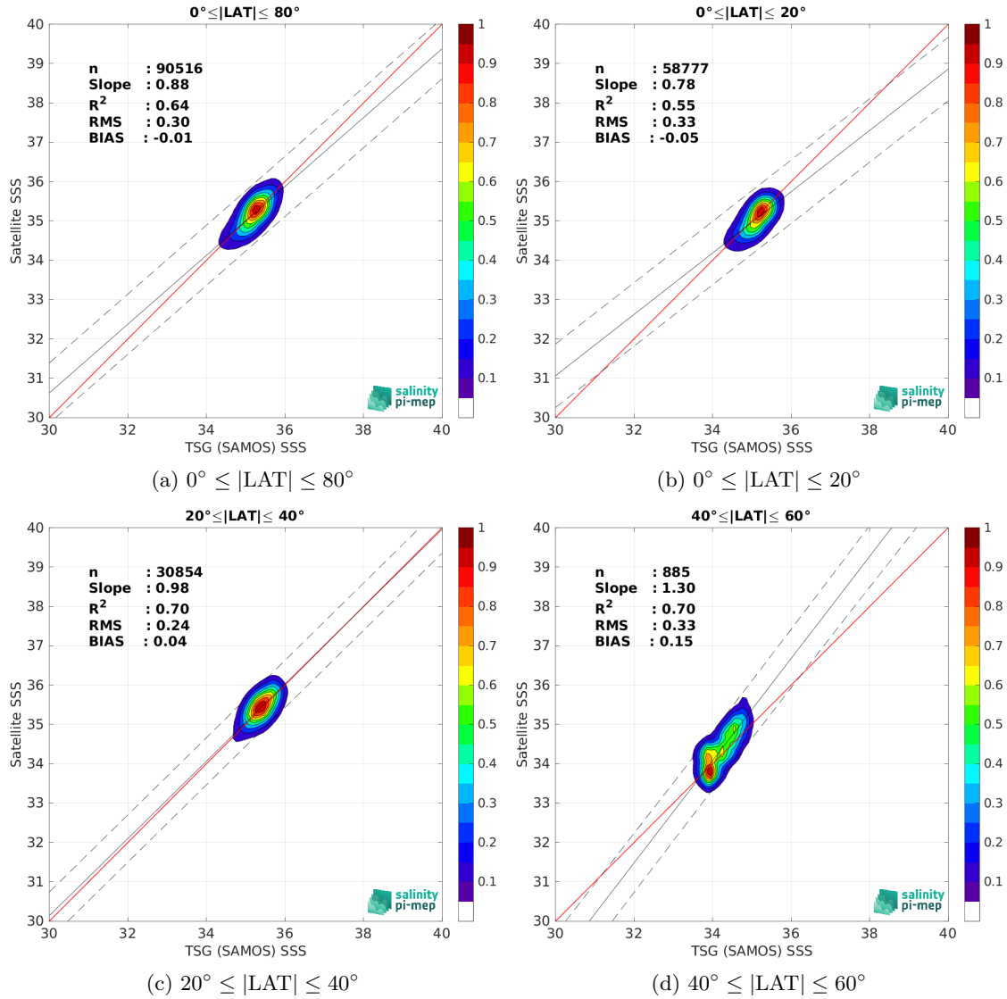
Figure 10: Contour maps of the concentration of SMAP SSS L3 v5.3 - 8-Day running (RSS) SSS (y-axis) versus TSG (SAMOS) SSS (x-axis) at match-up pairs for different latitude bands. For each plot, the red line shows x=y . The black thin and dashed lines indicate a linear fit through the data cloud and the \pm 95\% confidence levels, respectively. The number match-up pairs n , the slope and R^2 coefficient of the linear fit, the root mean square (RMS) and the mean bias between satellite and in situ data are indicated for each latitude band in each plots.
