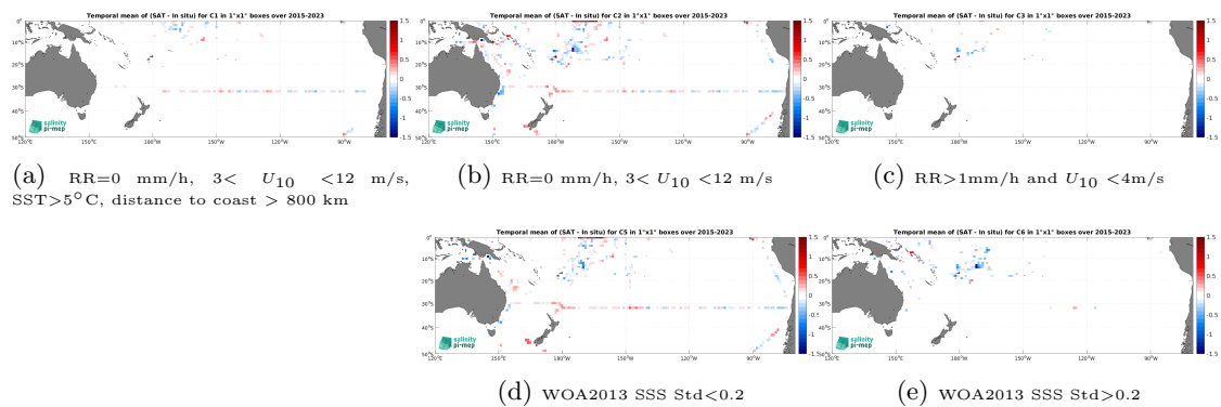
Figure 14: Temporal mean gridded over spatial boxes of size 1^\circ \times 1^\circ of \Delta SSS (SMAP SSS L3 v5.3 - 8-Day running (RSS) - TSG (SAMOS)) for 5 different subdatasets corresponding to: RR=0 mm/h, 3 < U_{10} < 12 m/s, SST > 5^\circ\text{C} , distance to coast > 800 km (a), RR=0 mm/h, 3 < U_{10} < 12 m/s (b), RR > 1 mm/h and U_{10} < 4 m/s (c), WOA2013 SSS Std < 0.2 (d), WOA2013 SSS Std > 0.2 (e).
