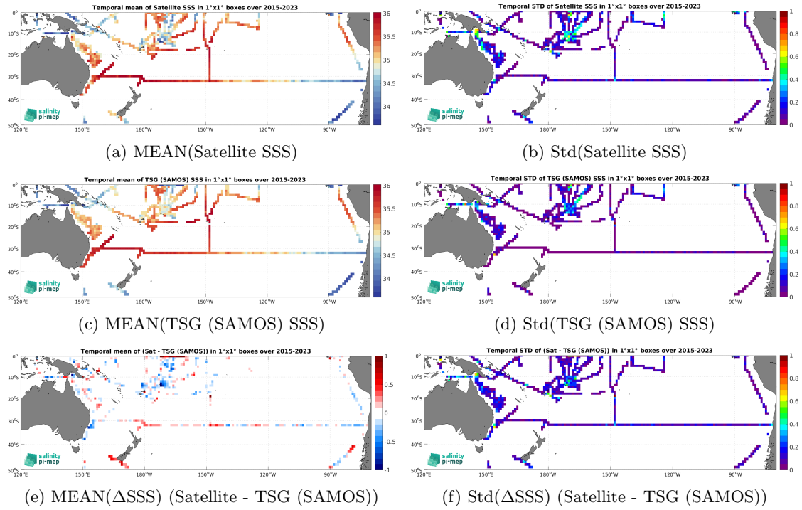
Figure 7: Temporal mean (left) and Std (right) of SSS from SMAP SSS L3 v5.3 - 8-Day running (RSS) (top), TSG (SAMOS) (middle), and of \Delta SSS (Satellite - TSG (SAMOS)). Only match-up pairs are used to generate these maps.
