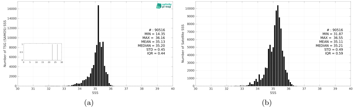
Figure 3: Histograms of SSS from TSG (SAMOS) (a) and SMAP SSS L3 v5.3 - 8-Day running (RSS) (b) considering all match-up pairs per bins of 0.1 over the South Pacific Ocean Pi-MEP region and for the full satellite product period.
