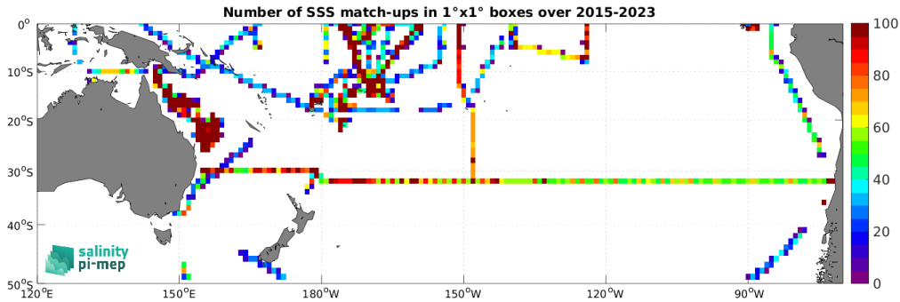
Figure 5: Number of SSS match-ups between TSG (SAMOS) SSS and the SMAP SSS L3 v5.3 - 8-Day running (RSS) SSS product for the South Pacific Ocean Pi-MEP region over 1^\circ \times 1^\circ boxes and for the full satellite product period.
