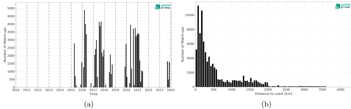
Figure 2: Number of match-ups between TSG (SAMOS) and SMAP SSS L3 v5.3 - 8-Day running (RSS) SSS as a function of time (a) and as function of the distance to coast (b) over the South Pacific Ocean Pi-MEP region and for the full satellite product period.
